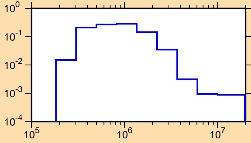
\sigma vs. E for ^{152}\text{Tb}(n,n_3)
