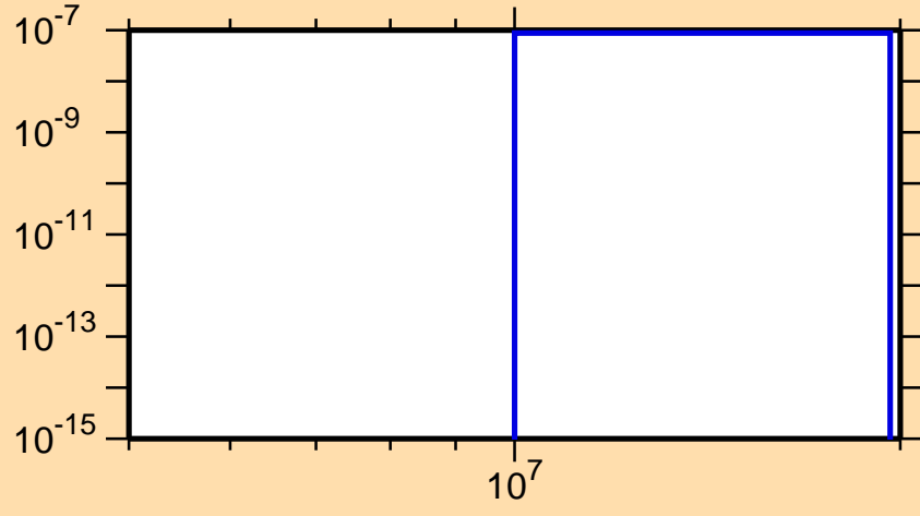
\sigma vs. E for ^{152}\text{Tb}(n,\text{He}3)
