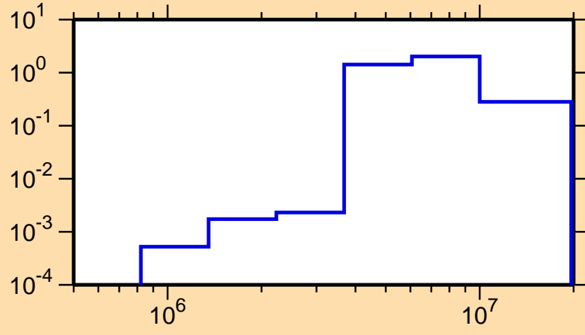
\sigma vs. E for ^{152}\text{Tb}(n,n\text{cont.})
