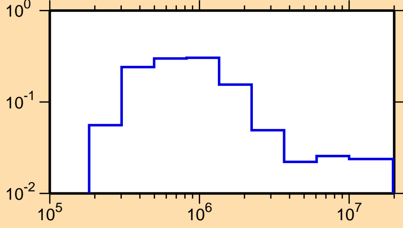
\sigma vs. E for ^{152}\text{Tb}(n,n_1)
