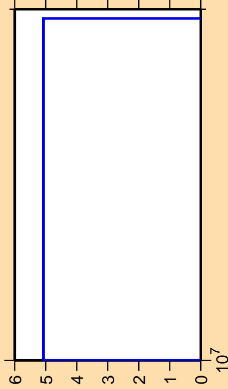
\Delta\sigma/\sigma vs. E for ^{152}\text{Tb} (mt 34)
