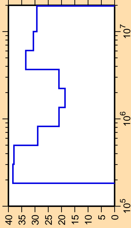
\Delta\sigma/\sigma vs. E for ^{152}\text{Tb}(n,n_1)
