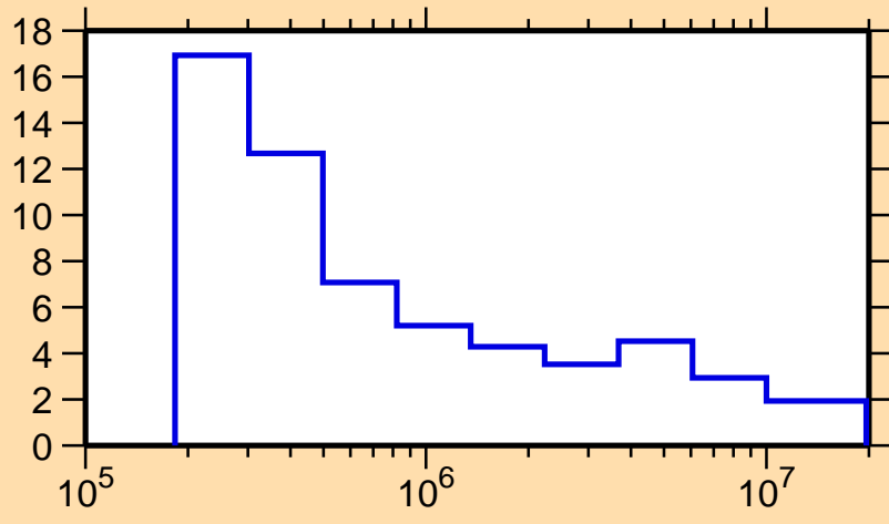
\Delta\sigma/\sigma vs. E for ^{152}\text{Tb}(n,\text{tot.})
