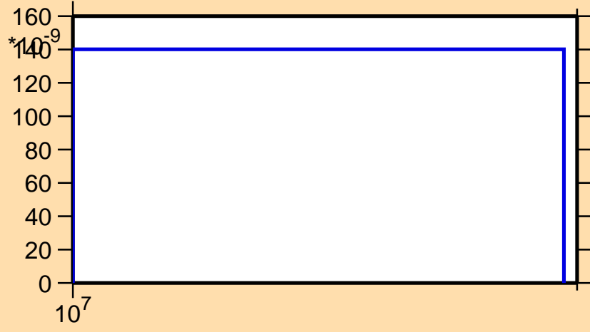
\sigma vs. E for ^{152}\text{Tb}(n,nt)
