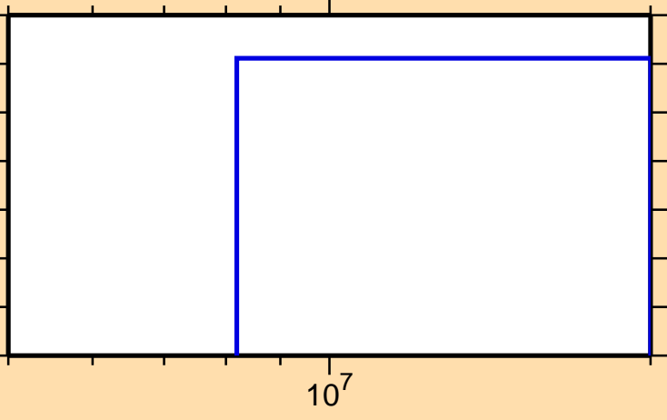
\sigma vs. E for ^{152}\text{Tb}(n,2n\alpha)
