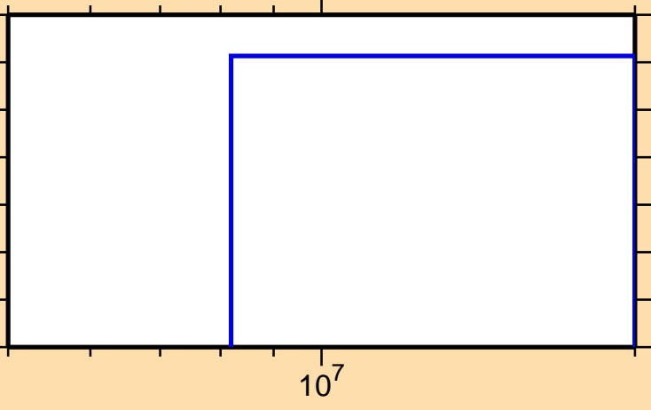
\sigma vs. E for ^{152}\text{Tb} (mt 42)
