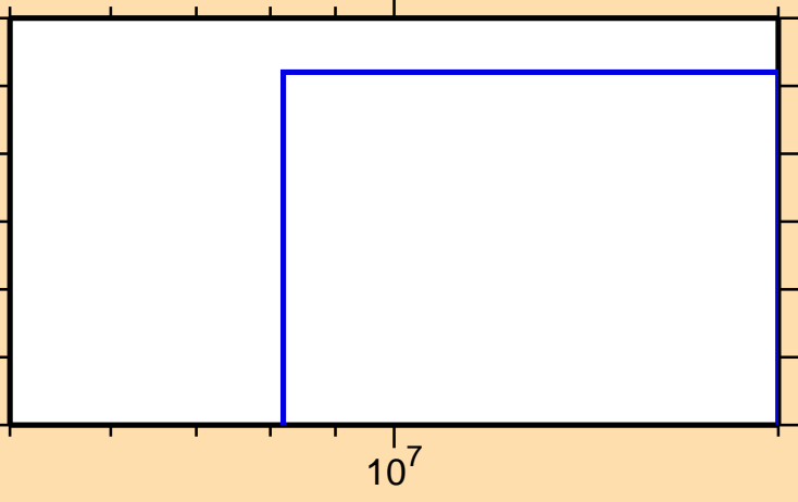
\sigma vs. E for ^{152}\text{Tb}(n,\text{nd})
