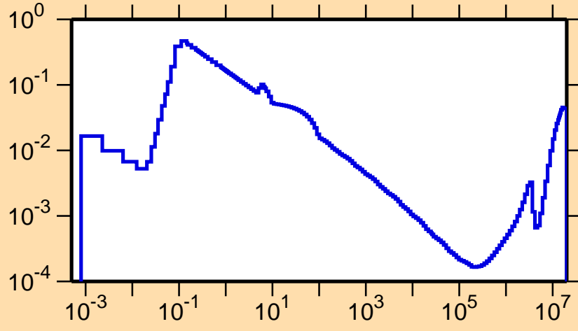
\sigma vs. E for ^{152}\text{Tb}(n,\alpha)
