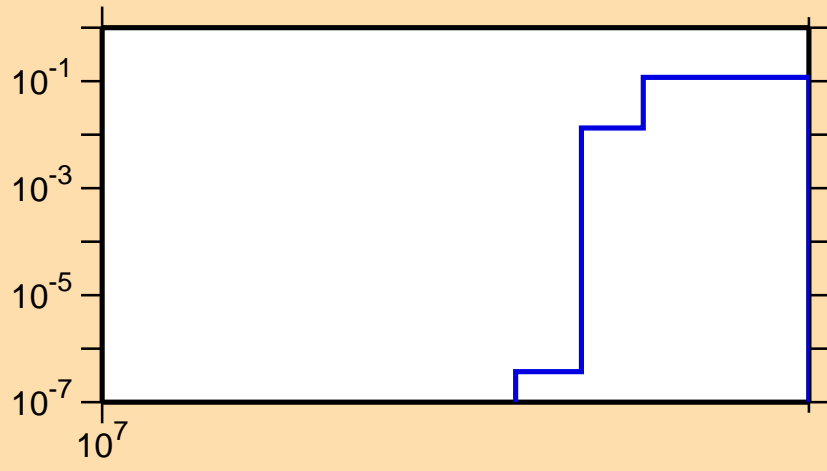
\sigma vs. E for ^{153}\text{Tb}(n,3n)
