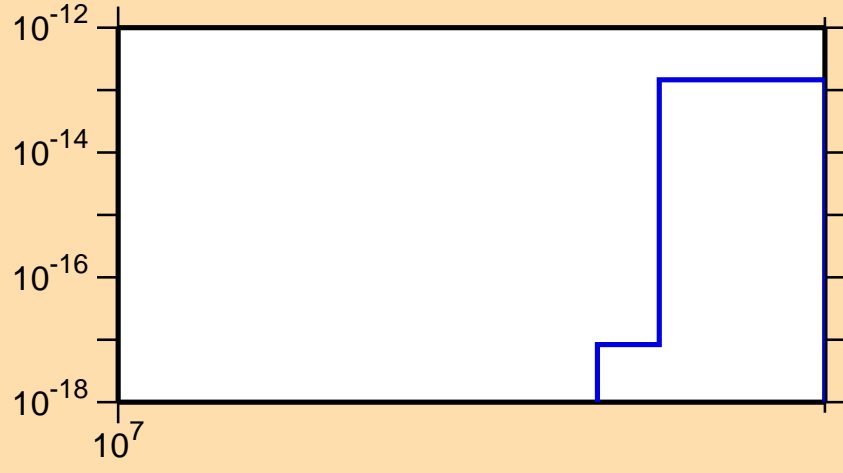
\sigma vs. E for ^{153}\text{Tb} (mt 34)
