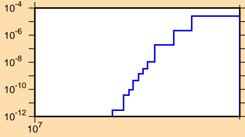
\sigma vs. E for ^{153}\text{Tb}(n,\text{nd})
