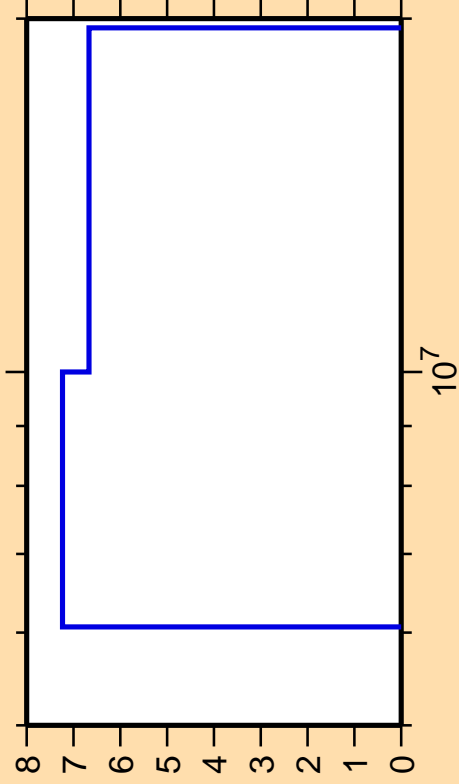
\Delta\sigma/\sigma vs. E for ^{153}\text{Tb}(n,2n)
