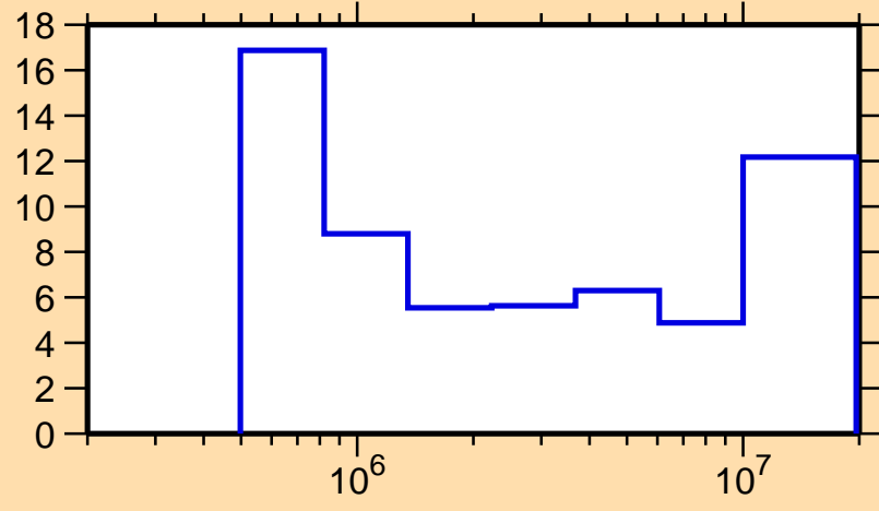
\Delta\sigma/\sigma vs. E for ^{153}\text{Tb}(n,\text{inel.})
