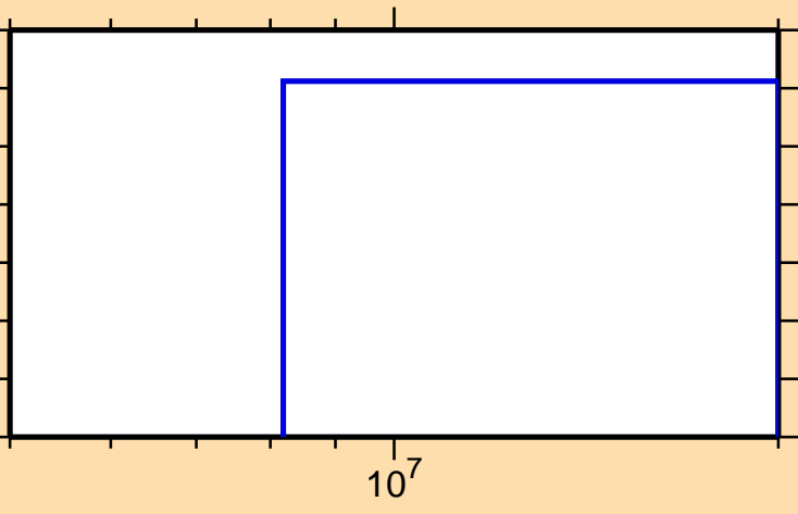
\sigma vs. E for ^{153}\text{Tb}(n,2np)
