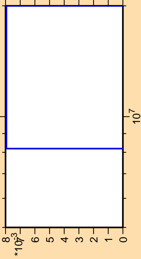
\Delta\sigma/\sigma vs. E for ^{153}\text{Tb} (mt 34)
