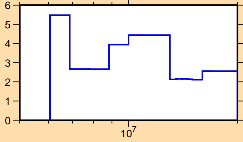
\Delta\sigma/\sigma vs. E for ^{154}\text{Tb}(n,\text{el.})
