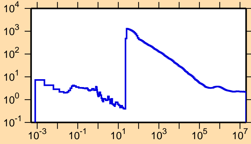
\sigma vs. E for ^{154}\text{Tb}(n,\text{nonel.})
