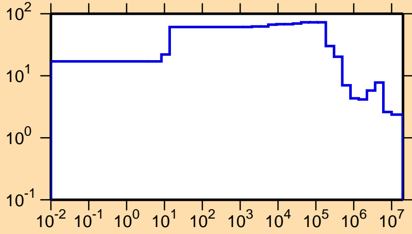
\Delta\sigma/\sigma vs. E for ^{154}\text{Tb}(n,el.)
