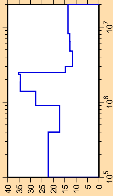
\Delta\sigma/\sigma vs. E for ^{155}\text{Tb}(n,n_2)
