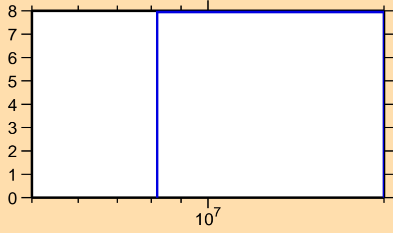
\Delta\sigma/\sigma vs. E for ^{155}\text{Tb}(n,\text{inel.})
