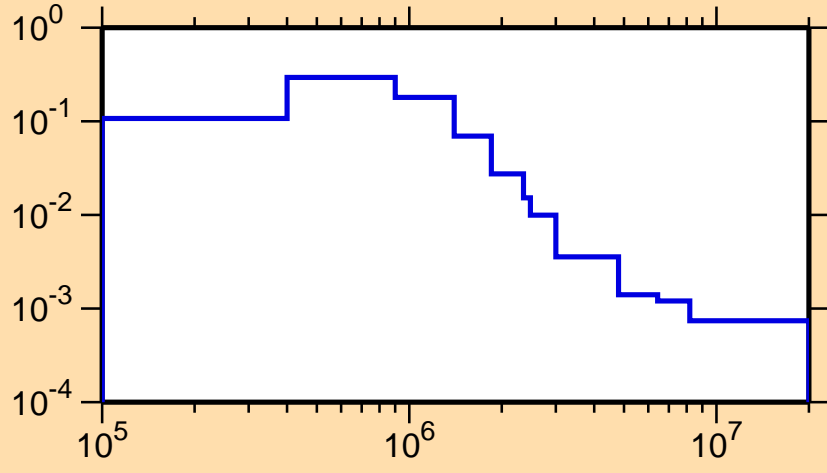
\sigma vs. E for ^{155}\text{Tb}(n,n_2)
