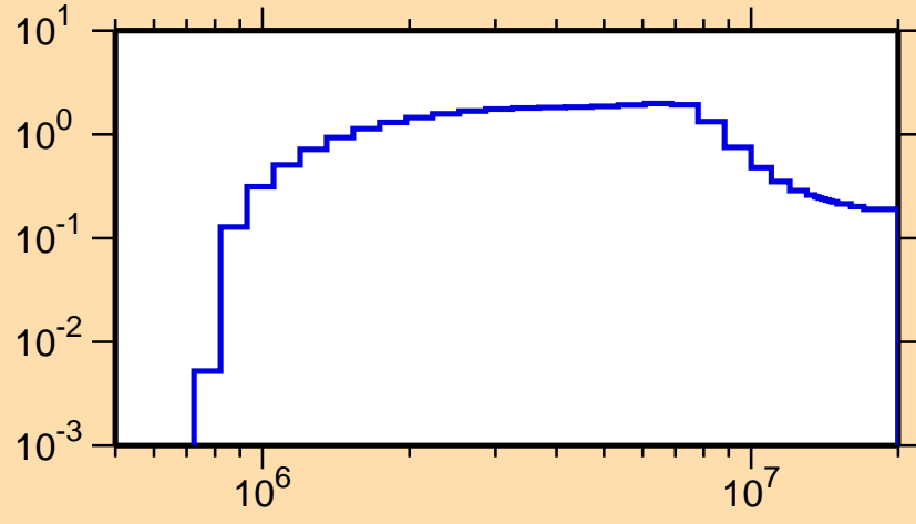
\sigma vs. E for ^{156}\text{Tb}(n,n\text{cont.})
