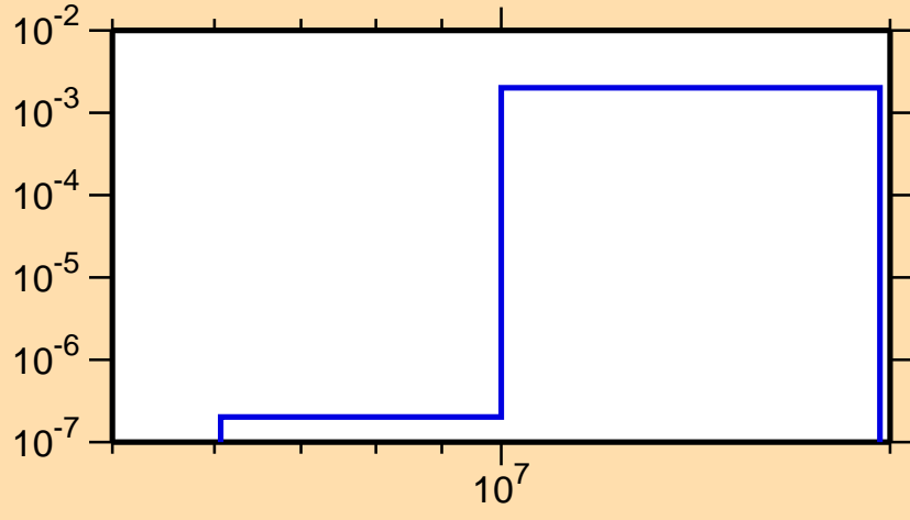
\sigma vs. E for ^{156}\text{Tb}(n,d)
