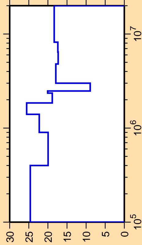
\Delta\sigma/\sigma vs. E for ^{156}\text{Tb}(n,n_4)
