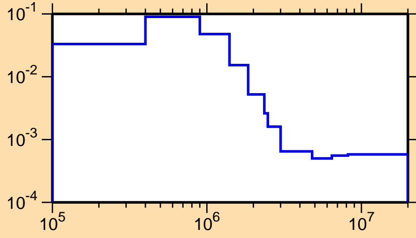
\sigma vs. E for ^{156}\text{Tb}(n,n_4)
