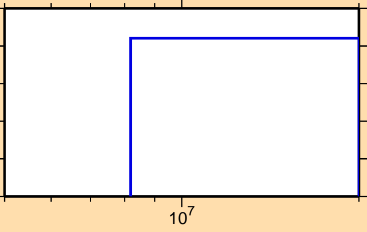
\sigma vs. E for ^{156}\text{Tb}(n,2np)
