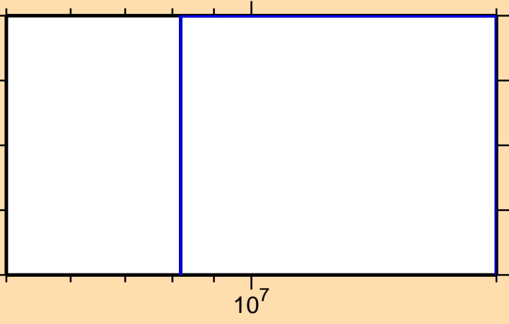
\sigma vs. E for ^{156}\text{Tb}(n,\text{nd})
