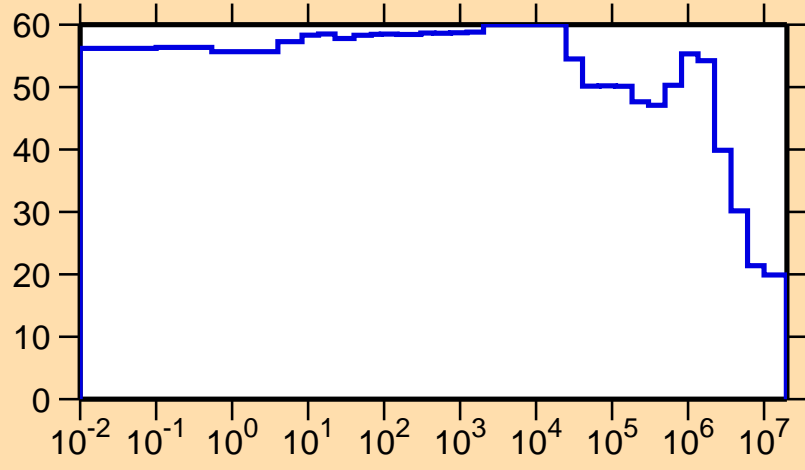
\Delta\sigma/\sigma vs. E for ^{156}\text{Tb}(n,p)
