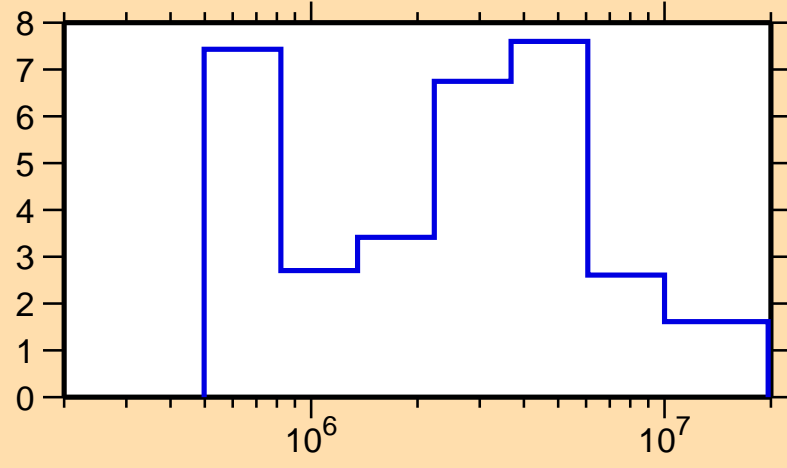
\Delta\sigma/\sigma vs. E for ^{156}\text{Tb}(n,\text{el.})
