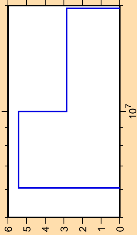
\Delta\sigma/\sigma vs. E for ^{156}\text{Tb}(n,2n)
