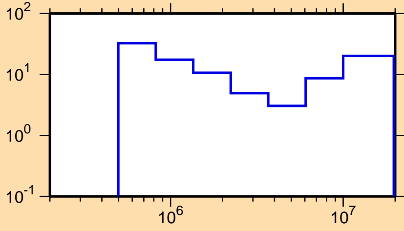
\Delta\sigma/\sigma vs. E for ^{156}\text{Tb}(n,n\text{cont.})
