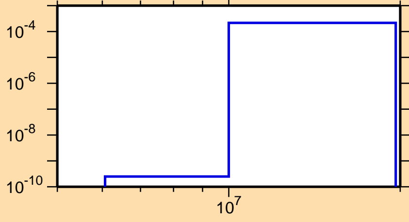
\sigma vs. E for ^{156}\text{Tb}(n,t)
