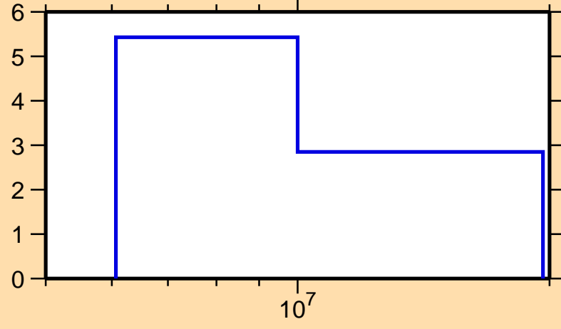
\Delta\sigma/\sigma vs. E for ^{156}\text{Tb}(n,2n)
