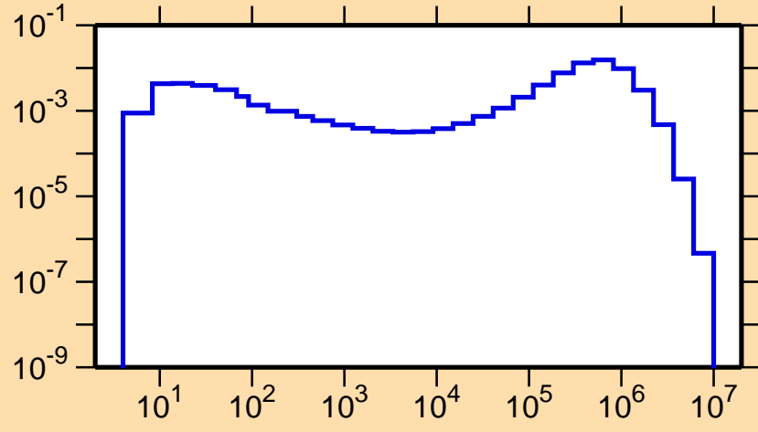
\sigma vs. E for ^{156}\text{Tb}(n,n_2)
