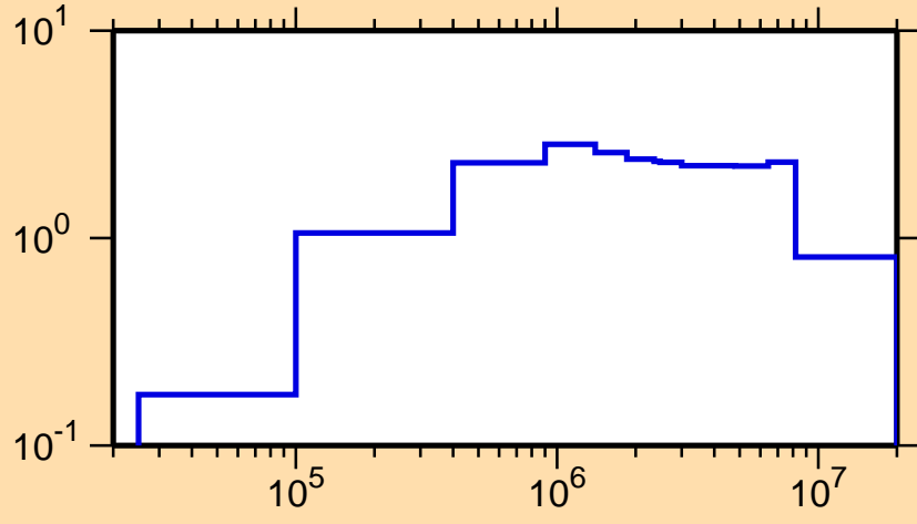
\sigma vs. E for ^{157}\text{Tb}(n,\text{inel.})
