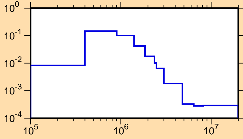
\sigma vs. E for ^{157}\text{Tb}(n,n_4)
