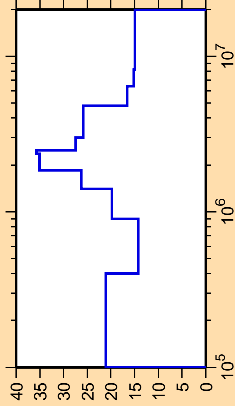
\Delta\sigma/\sigma vs. E for ^{157}\text{Tb}(n,n_2)
