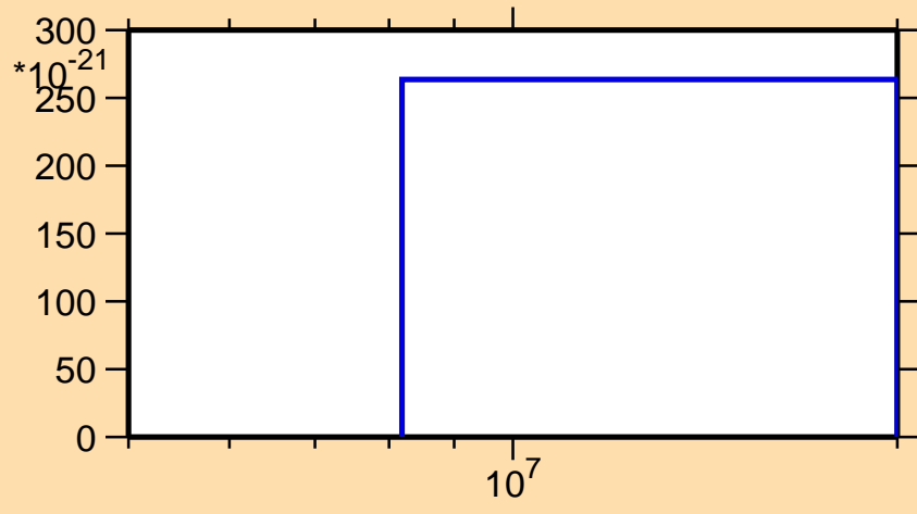
\sigma vs. E for ^{157}\text{Tb}(\text{mt } 11)
