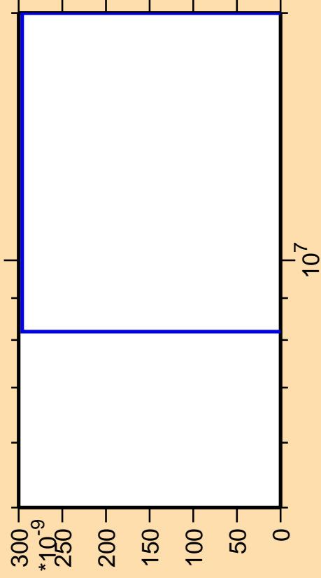
\Delta\sigma/\sigma vs. E for ^{157}\text{Tb}(\text{mt } 11)
