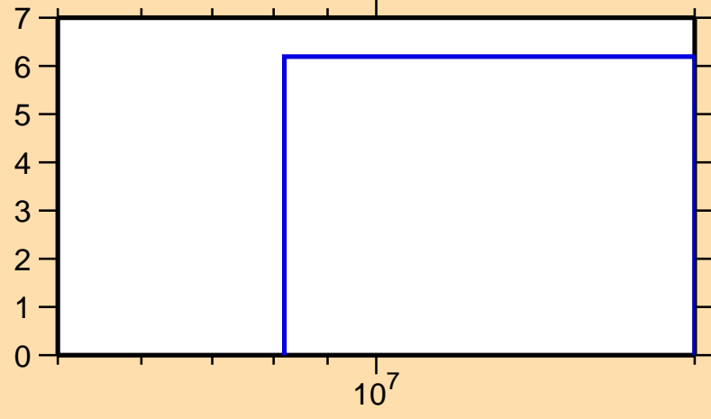
\Delta\sigma/\sigma vs. E for ^{157}\text{Tb}(n,\text{inel.})
