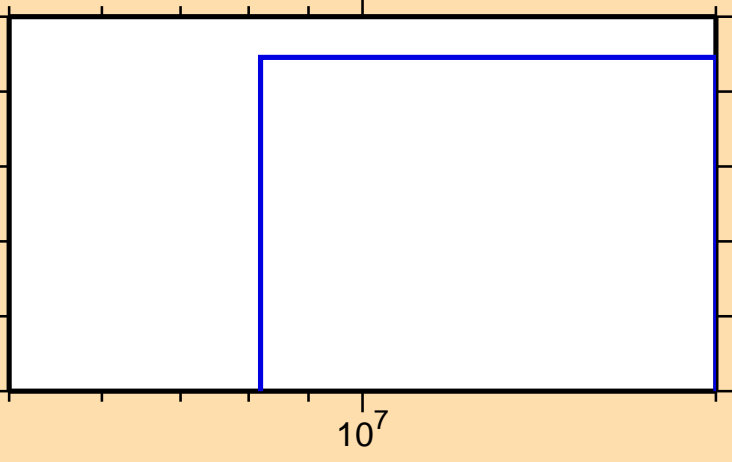
\sigma vs. E for ^{157}\text{Tb}(n,2np)
