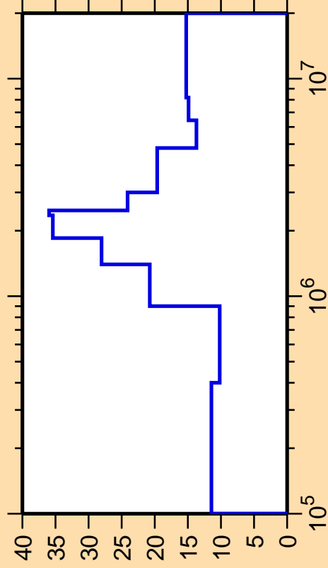
\Delta\sigma/\sigma vs. E for ^{157}\text{Tb}(n,n_4)
