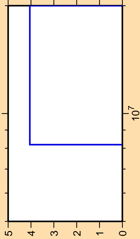
\Delta\sigma/\sigma vs. E for ^{157}\text{Tb}(n,2n)
