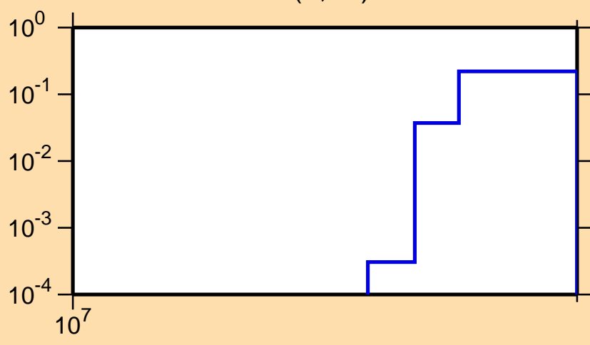
\sigma vs. E for ^{158}\text{Tb}(n,3n)
