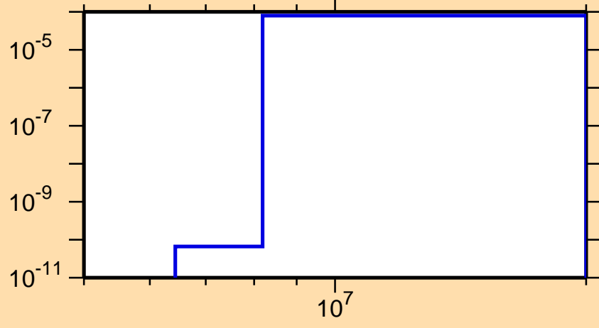
\sigma vs. E for ^{158}\text{Tb}(n,n\alpha)
