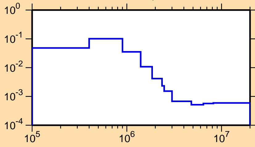
\sigma vs. E for ^{158}\text{Tb}(n,n_4)
