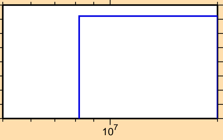
\sigma vs. E for ^{158}\text{Tb}(n,2np)
