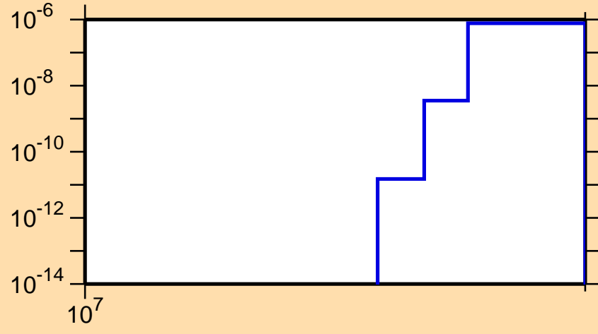
\sigma vs. E for ^{159}\text{Tb}(n,nt)
