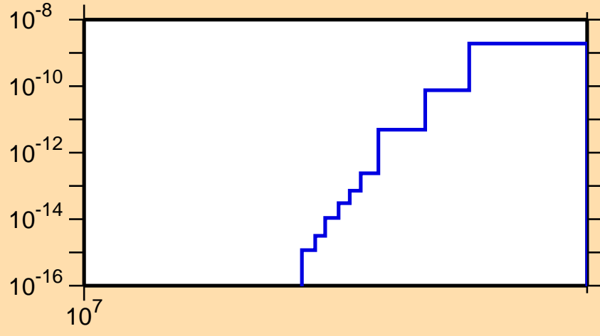
\sigma vs. E for ^{159}\text{Tb}(n,\text{He3})
