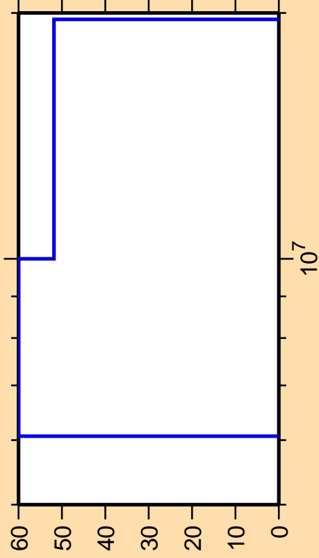
\Delta\sigma/\sigma vs. E for ^{159}\text{Tb}(n,n\alpha)
