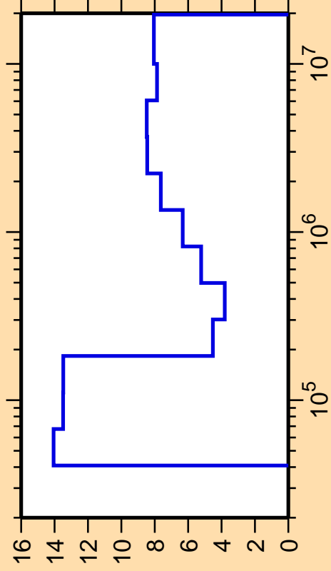
\Delta\sigma/\sigma vs. E for ^{159}\text{Tb}(n,n_1)
