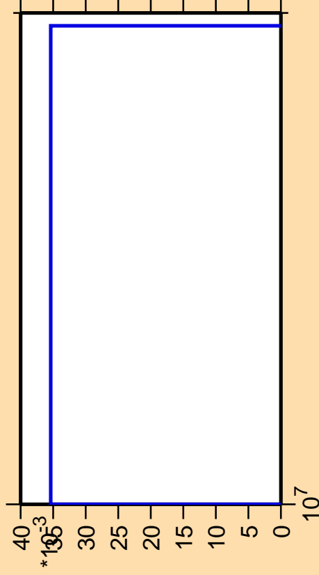
\Delta\sigma/\sigma vs. E for ^{159}\text{Tb}(n,p\alpha)
