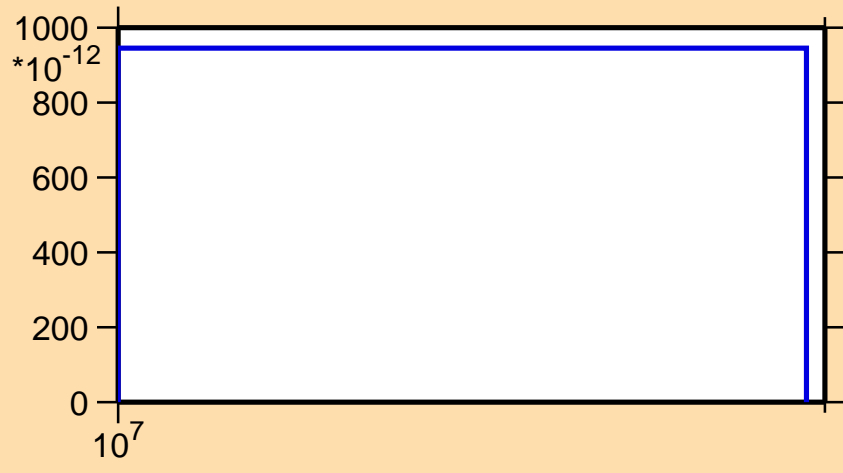
\sigma vs. E for ^{159}\text{Tb}(n,2np)
