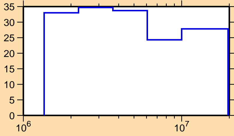
\Delta\sigma/\sigma vs. E for ^{159}\text{Tb}(n,\gamma)
