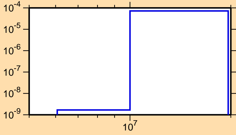
\sigma vs. E for ^{159}\text{Tb}(n,n\alpha)
