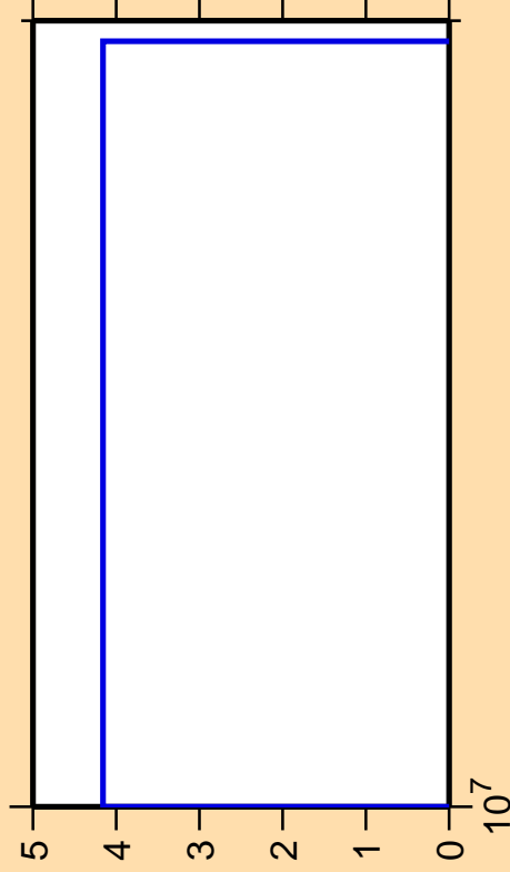
\Delta\sigma/\sigma vs. E for ^{159}\text{Tb}(n,3n)
