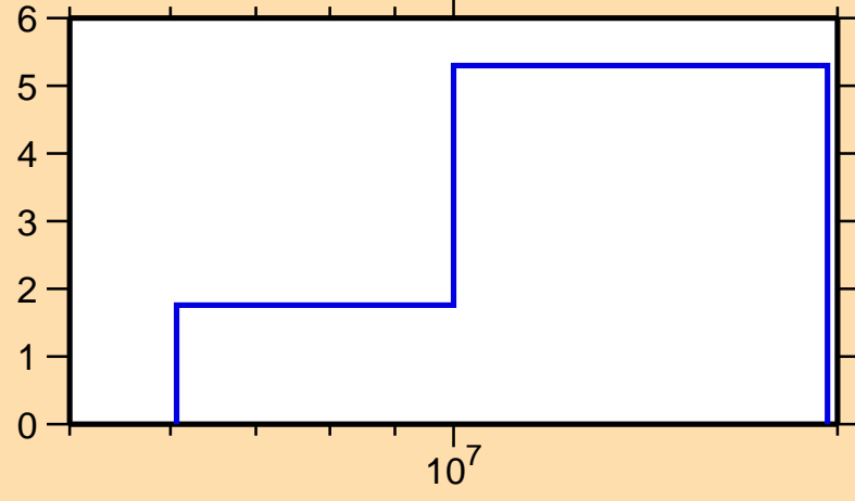
\Delta\sigma/\sigma vs. E for ^{159}\text{Tb}(n,\text{inel.})
