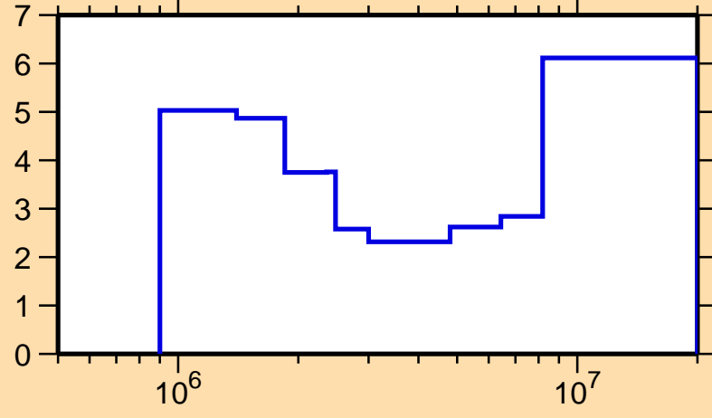
\Delta\sigma/\sigma vs. E for ^{159}\text{Tb}(n,n\text{cont.})
