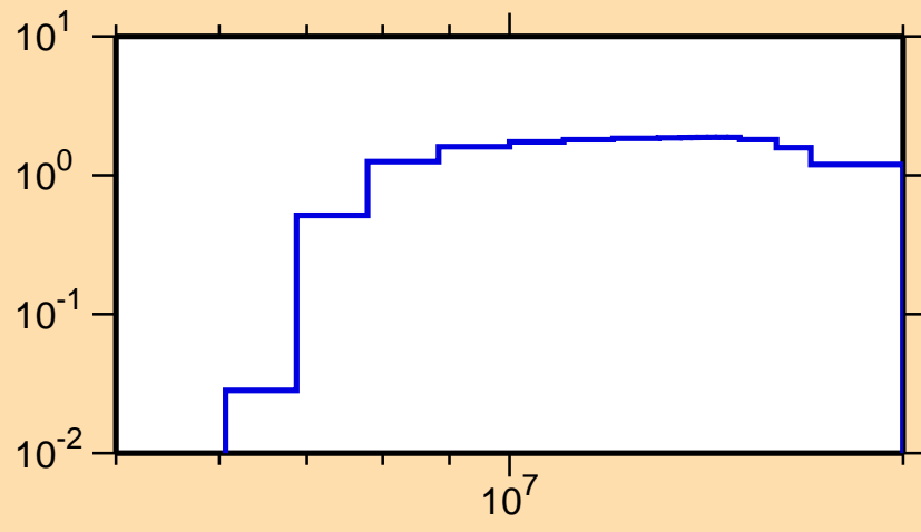
\sigma vs. E for ^{160}\text{Tb}(n,2n)
