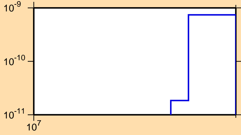
\sigma vs. E for ^{160}\text{Tb}(n,\text{He3})
