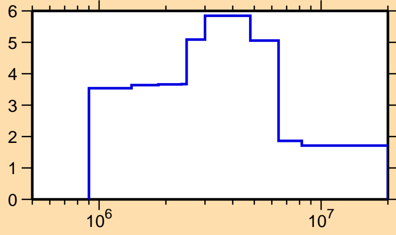
\Delta\sigma/\sigma vs. E for ^{160}\text{Tb}(n,\text{el.})
