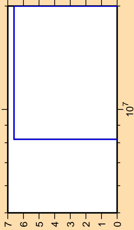
\Delta\sigma/\sigma vs. E for ^{160}\text{Tb}(n,3n)
