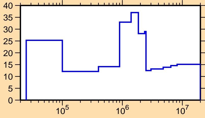
\Delta\sigma/\sigma vs. E for ^{160}\text{Tb}(n,n_1)
