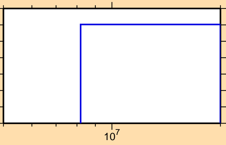
\sigma vs. E for ^{160}\text{Tb}(n,nt)
