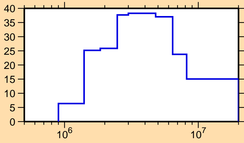
\Delta\sigma/\sigma vs. E for ^{160}\text{Tb}(n,p)
