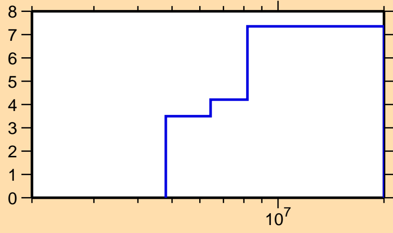
\Delta\sigma/\sigma vs. E for ^{160}\text{Tb}(n,\text{inel.})
