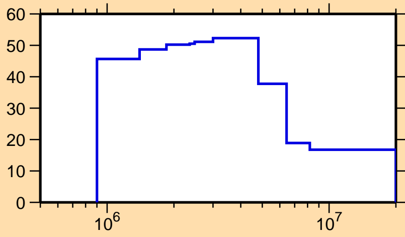
\Delta\sigma/\sigma vs. E for ^{160}\text{Tb}(n,\gamma)
