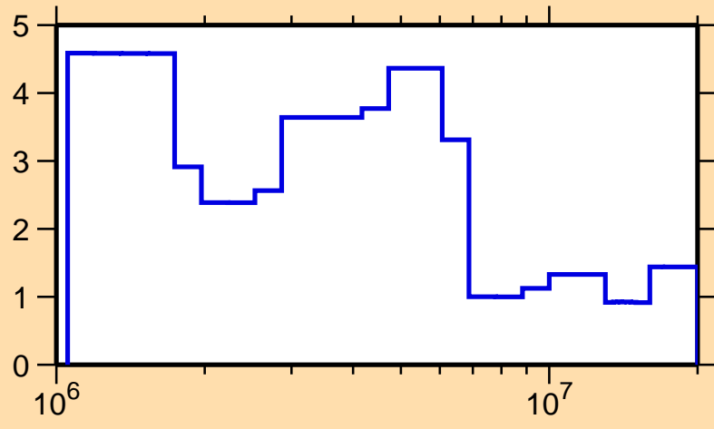
\Delta\sigma/\sigma vs. E for ^{161}\text{Tb}(n, tot.)
