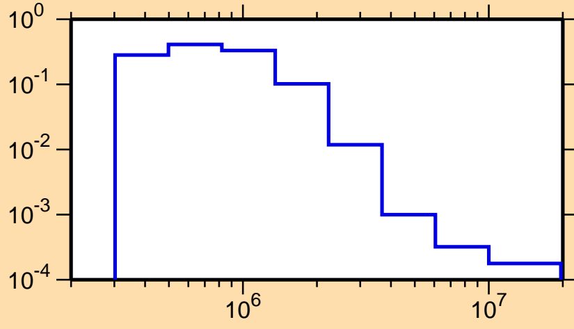
\sigma vs. E for ^{161}\text{Tb}(n,n_4)
