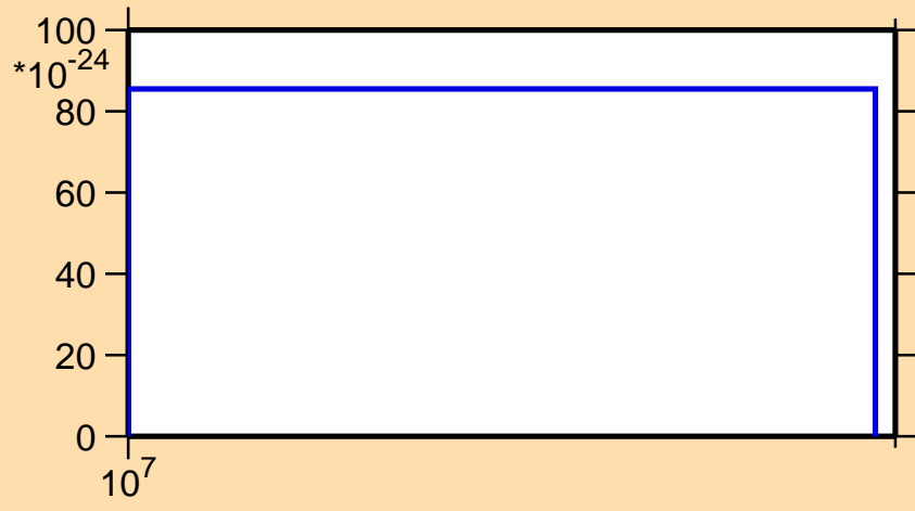
\sigma vs. E for ^{161}\text{Tb} (mt 11)
