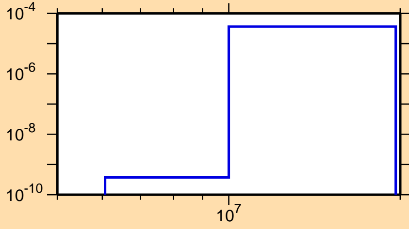
\sigma vs. E for ^{161}\text{Tb}(n,\alpha)
