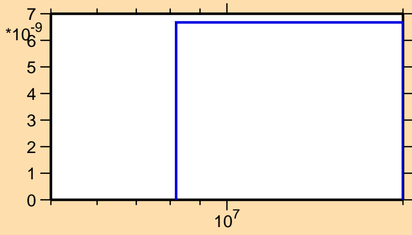
\sigma vs. E for ^{161}\text{Tb}(n,nt)
