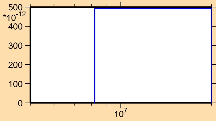
\sigma vs. E for ^{161}\text{Tb}(n,2np)
