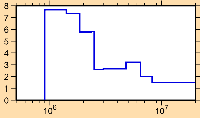
\Delta\sigma/\sigma vs. E for ^{161}\text{Tb}(n,\text{nonel.})
