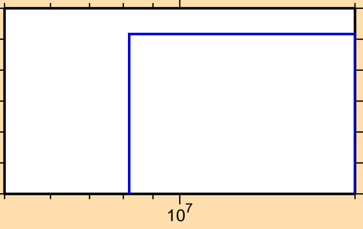
\sigma vs. E for ^{161}\text{Tb}(n,\text{nd})
