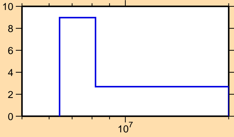
\Delta\sigma/\sigma vs. E for ^{161}\text{Tb}(n,2n)
