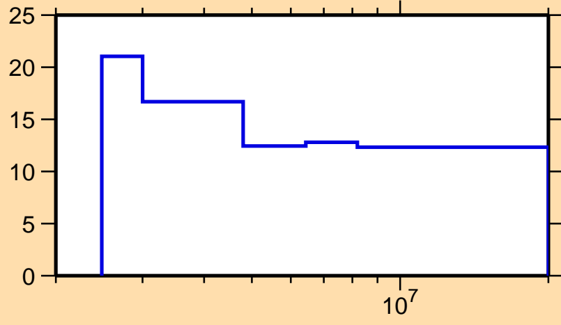
\Delta\sigma/\sigma vs. E for ^{161}\text{Tb}(n,n_1)
