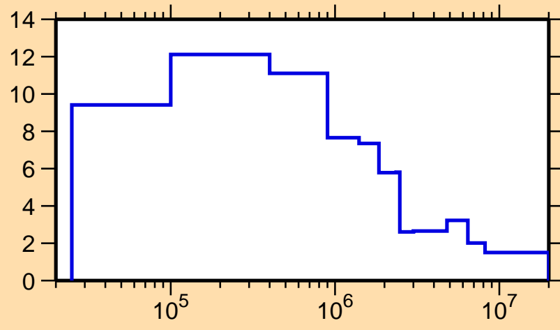
\Delta\sigma/\sigma vs. E for ^{161}\text{Tb}(n,\text{nonel.})
