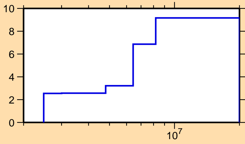
\Delta\sigma/\sigma vs. E for ^{161}\text{Tb}(n,n\text{cont.})
