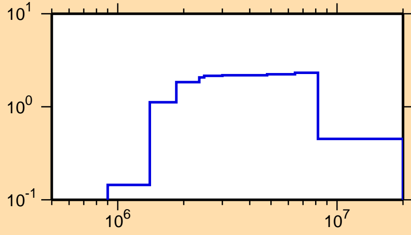
\sigma vs. E for ^{161}\text{Tb}(n,n\text{cont.})
