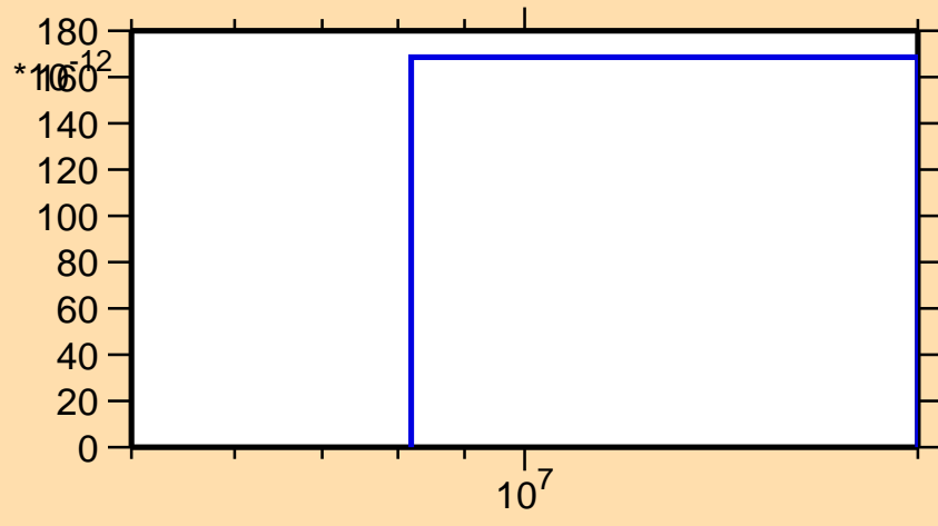
\sigma vs. E for ^{161}\text{Tb}(n,2n\alpha)
