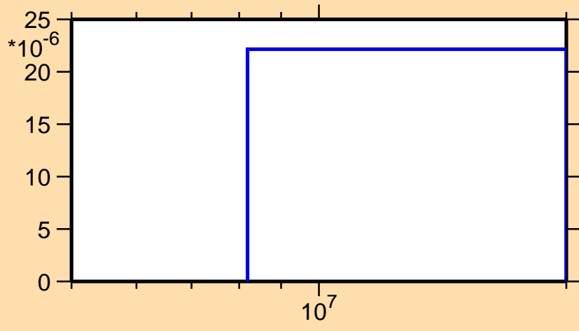
\sigma vs. E for ^{161}\text{Tb}(n,t)
