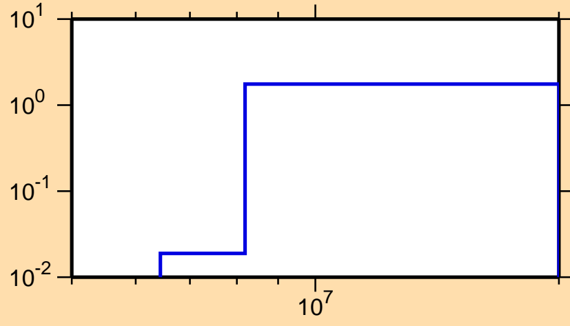
\sigma vs. E for ^{161}\text{Tb}(n,2n)
