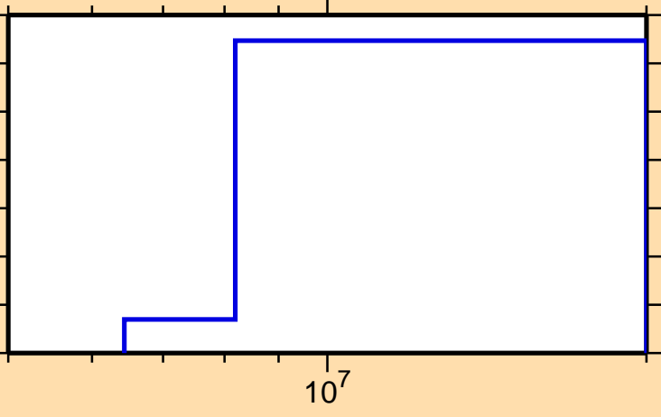
\sigma vs. E for ^{161}\text{Tb}(n,n\alpha)
