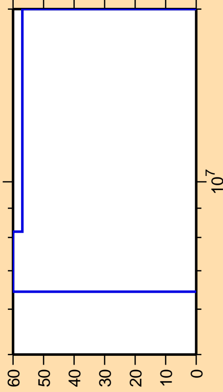
\Delta\sigma/\sigma vs. E for ^{161}\text{Tb}(n,n\alpha)
