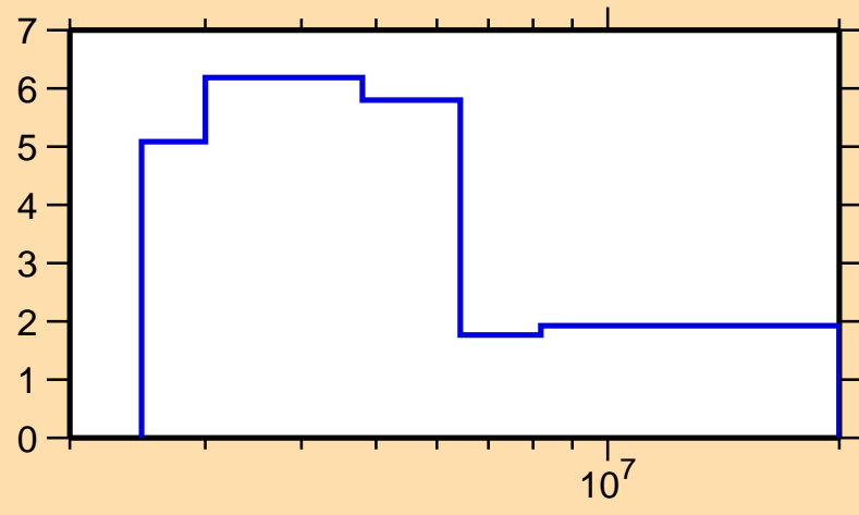
\Delta\sigma/\sigma vs. E for ^{161}\text{Tb}(n,\text{el.})
