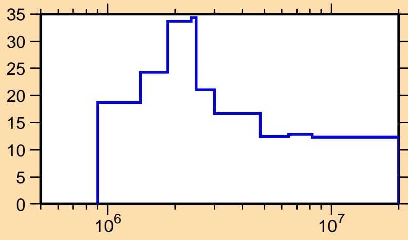
\Delta\sigma/\sigma vs. E for ^{161}\text{Tb}(n,n_1)
