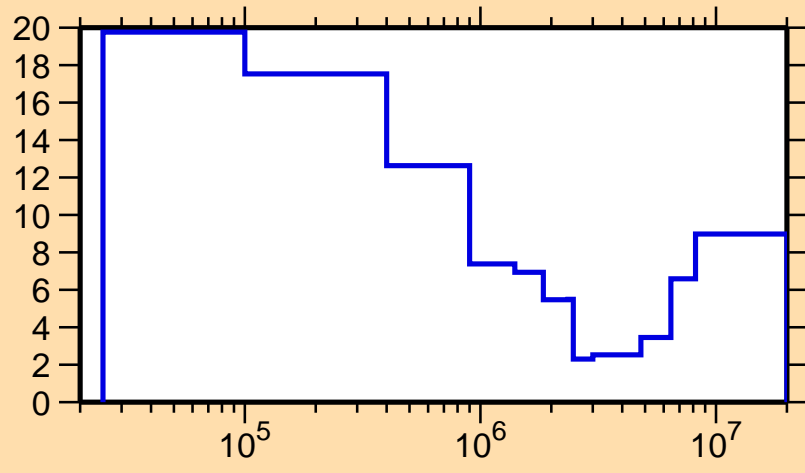
\Delta\sigma/\sigma vs. E for ^{161}\text{Tb}(n,\text{inel.})
