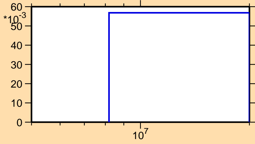
\sigma vs. E for ^{161}\text{Tb}(n,3n)
