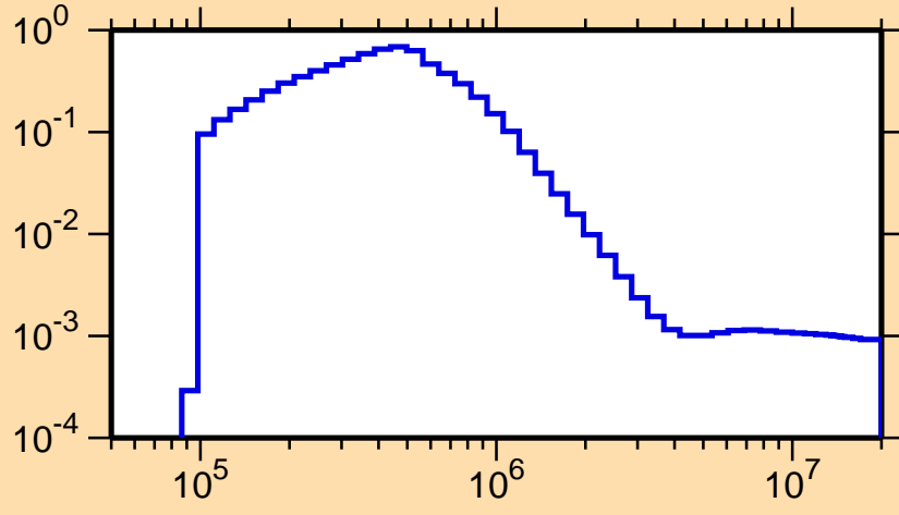
\sigma vs. E for ^{162}\text{Tb}(n,n_2)
