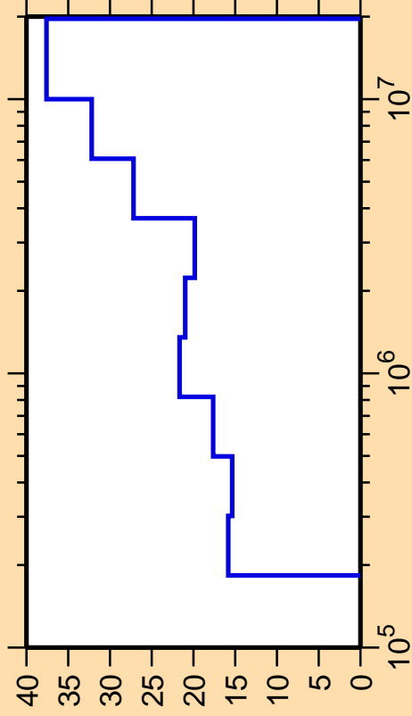
\Delta\sigma/\sigma vs. E for ^{162}\text{Tb}(n,n_4)
