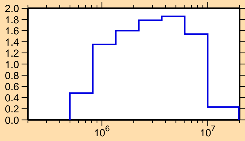
\sigma vs. E for ^{162}\text{Tb}(n,n\text{cont.})
