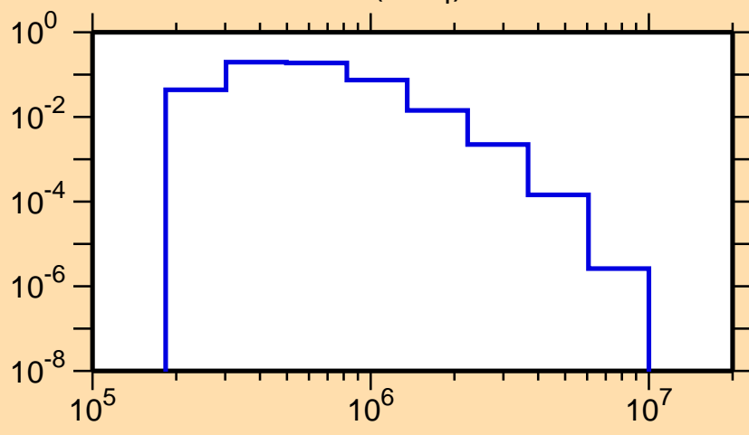
\sigma vs. E for ^{162}\text{Tb}(n,n_4)
