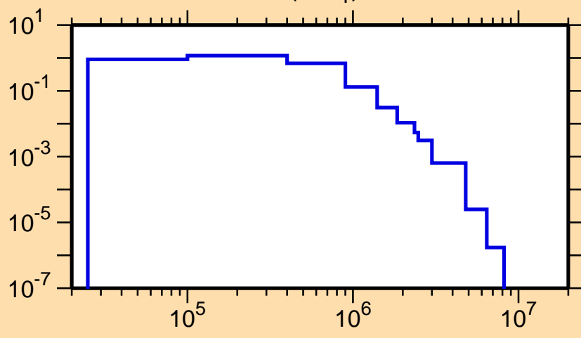
\sigma vs. E for ^{162}\text{Tb}(n,n_1)
