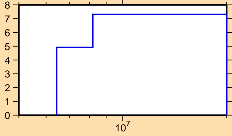
\Delta\sigma/\sigma vs. E for ^{162}\text{Tb}(n,\text{inel.})
