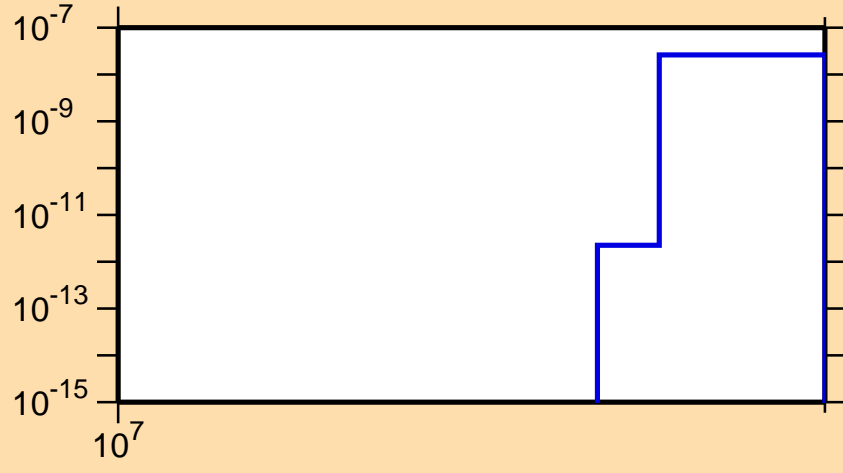
\sigma vs. E for ^{163}\text{Tb}(n,2np)
