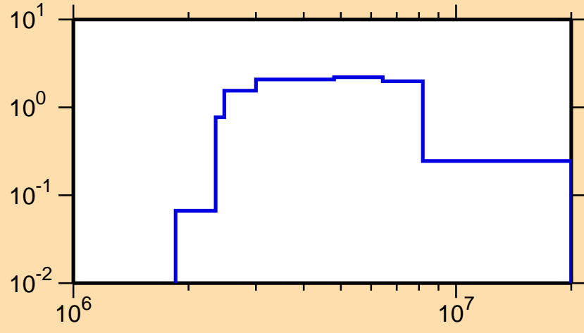
\sigma vs. E for ^{163}\text{Tb}(n,n\text{cont.})
