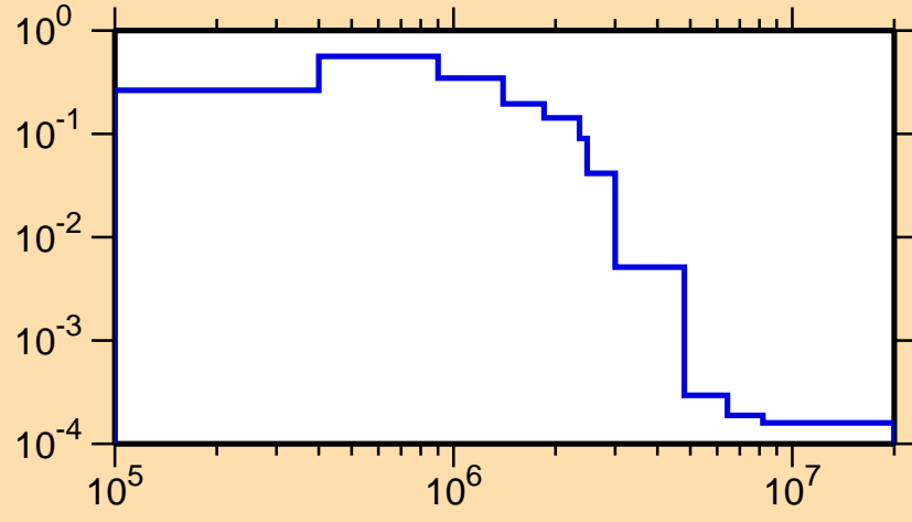
\sigma vs. E for ^{163}\text{Tb}(n,n_2)
