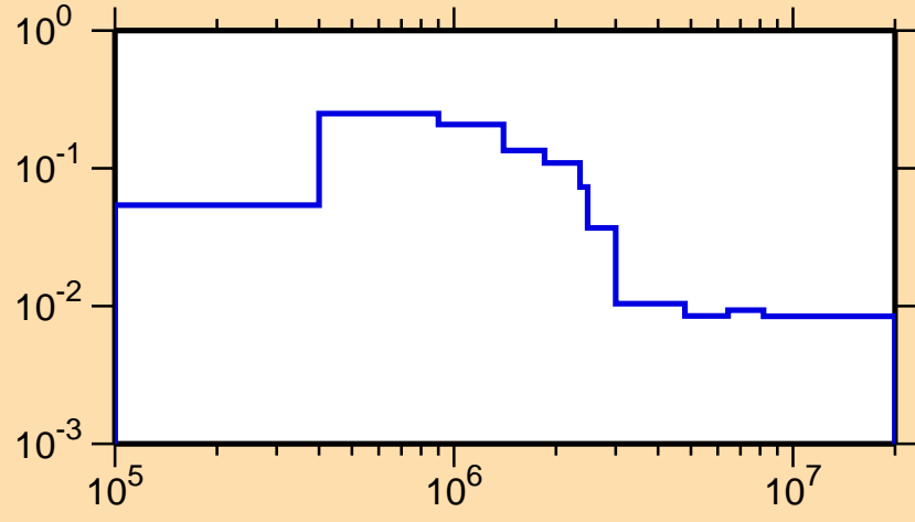
\sigma vs. E for ^{163}\text{Tb}(n,n_3)
