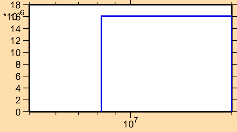
\sigma vs. E for ^{163}\text{Tb}(n,t)
