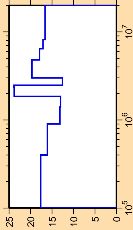
\Delta\sigma/\sigma vs. E for ^{163}\text{Tb}(n,n_3)
