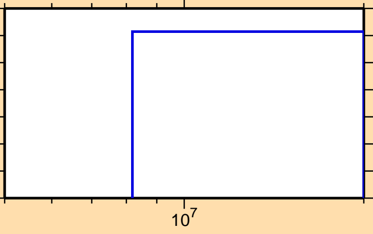
\sigma vs. E for ^{164}\text{Tb}(n,d)
