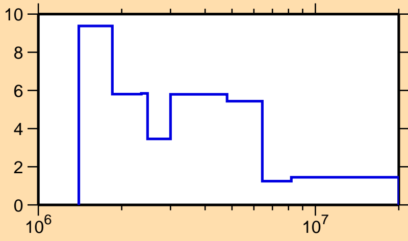
\Delta\sigma/\sigma vs. E for ^{164}\text{Tb}(n,\text{tot.})
