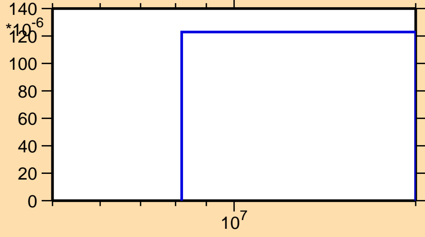
\sigma vs. E for ^{164}\text{Tb}(n,d)
