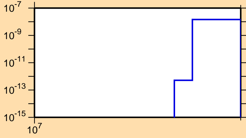
\sigma vs. E for ^{165}\text{Tb}(n,2np)
