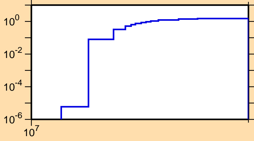
\sigma vs. E for ^{166}\text{Tb}(n,3n)
