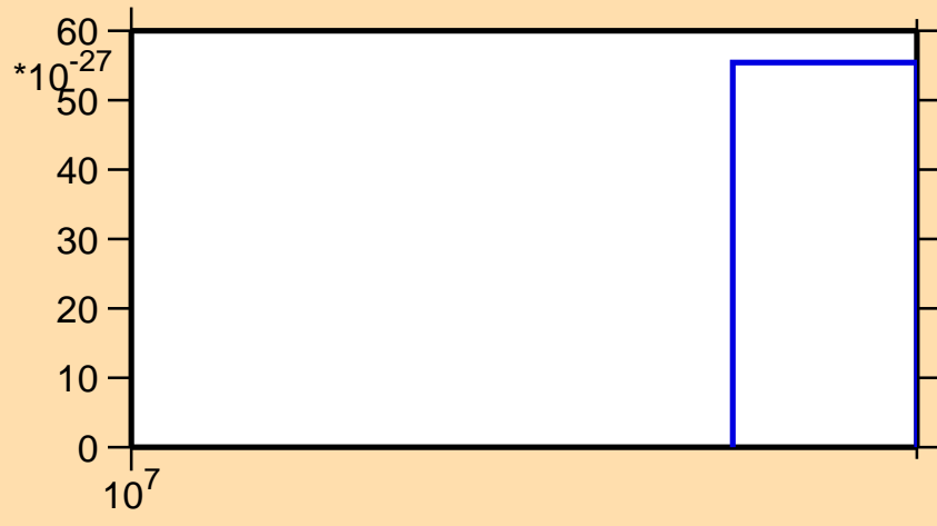
\sigma vs. E for ^{166}\text{Tb} (mt 42)
