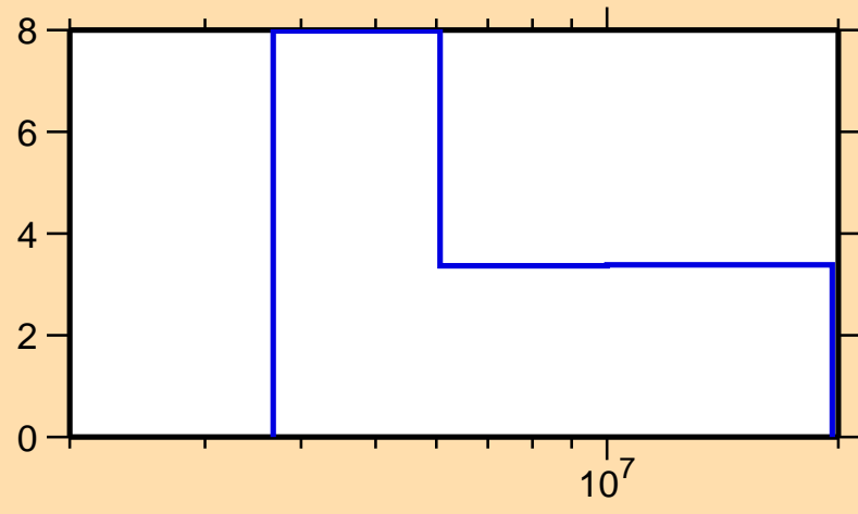
\Delta\sigma/\sigma vs. E for ^{166}\text{Tb}(n,\text{tot.})
