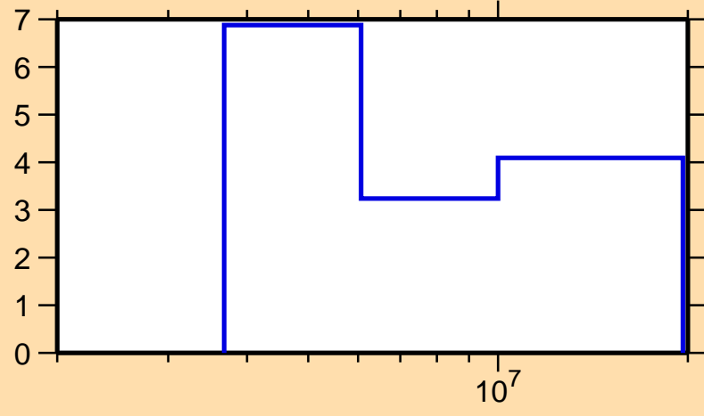
\Delta\sigma/\sigma vs. E for ^{166}\text{Tb}(n,\text{nonel.})
