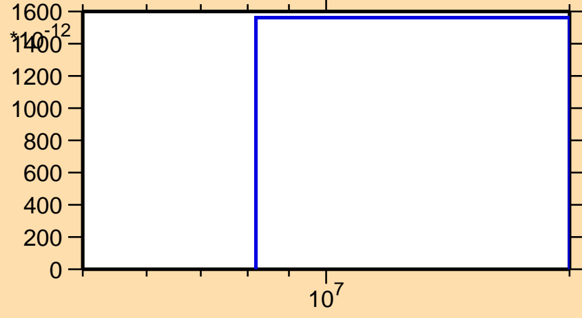
\sigma vs. E for ^{166}\text{Tb}(n,2np)
