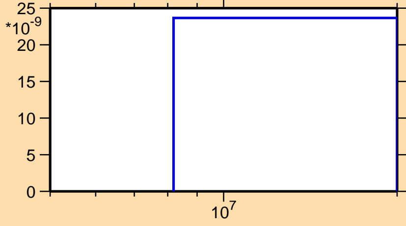
\sigma vs. E for ^{166}\text{Tb}(n,nt)
