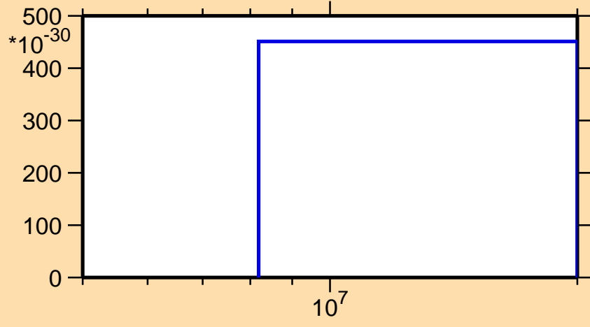
\sigma vs. E for ^{166}\text{Tb} (mt 42)
