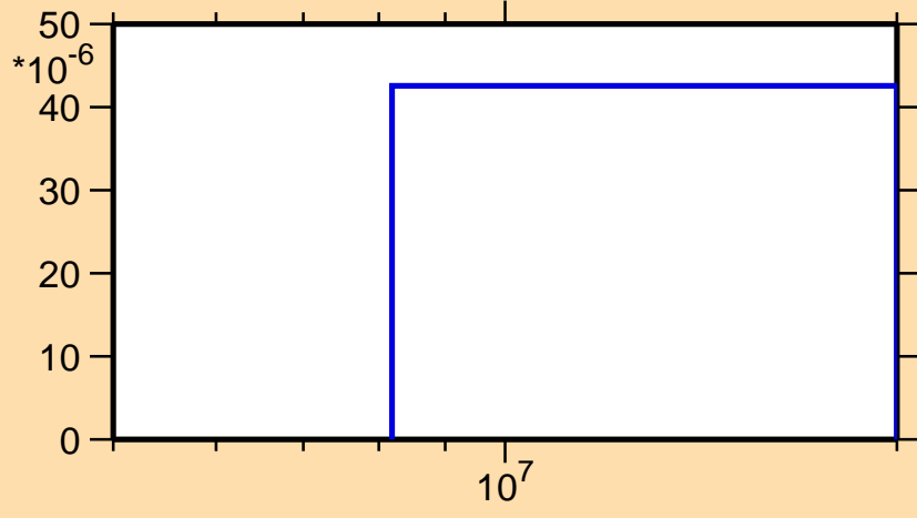
\sigma vs. E for ^{166}\text{Tb}(n,np)
