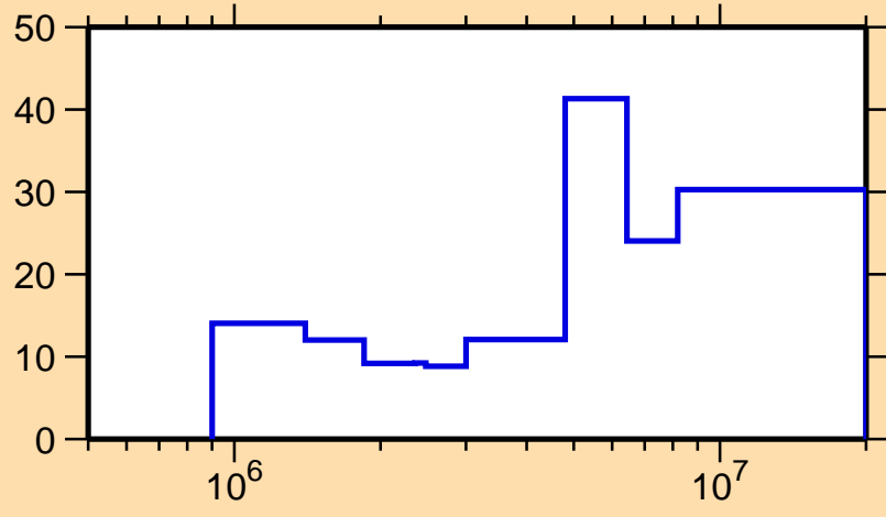
\Delta\sigma/\sigma vs. E for ^{166}\text{Tb}(n,\text{inel.})
