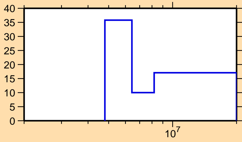
\Delta\sigma/\sigma vs. E for ^{166}\text{Tb}(n,2n)
