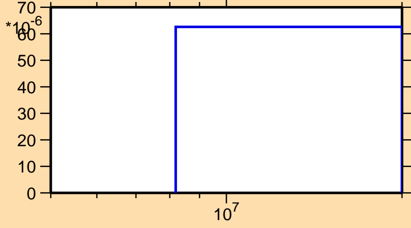
\sigma vs. E for ^{166}\text{Tb}(n,d)
