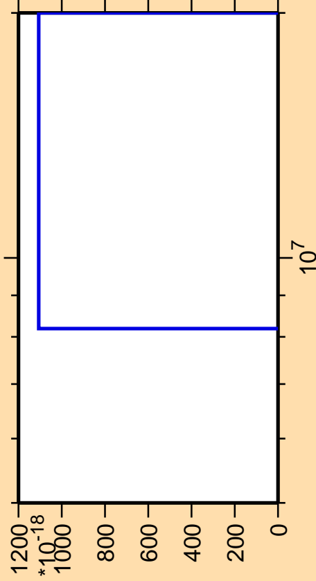
\Delta\sigma/\sigma vs. E for ^{166}\text{Tb} (mt 42)
