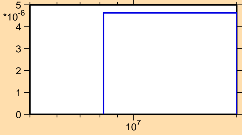
\sigma vs. E for ^{166}\text{Tb}(n,n\alpha)
