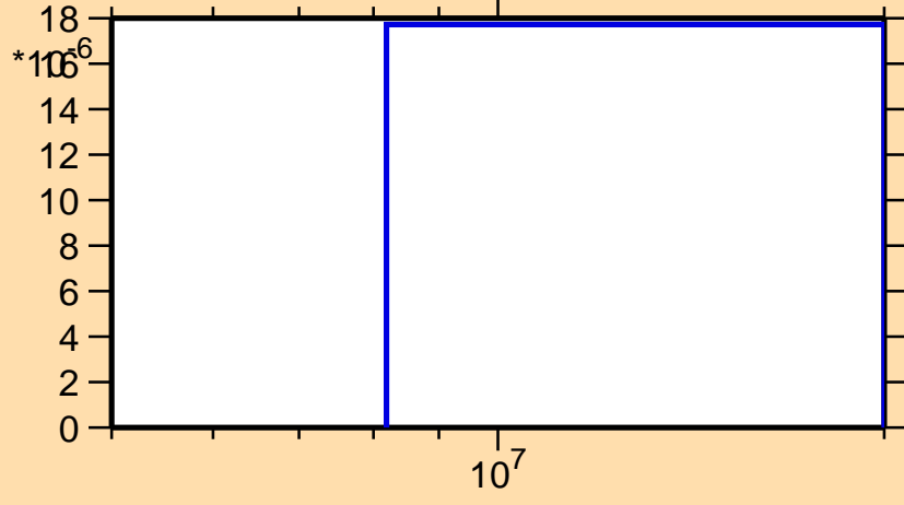
\sigma vs. E for ^{166}\text{Tb}(n,t)
