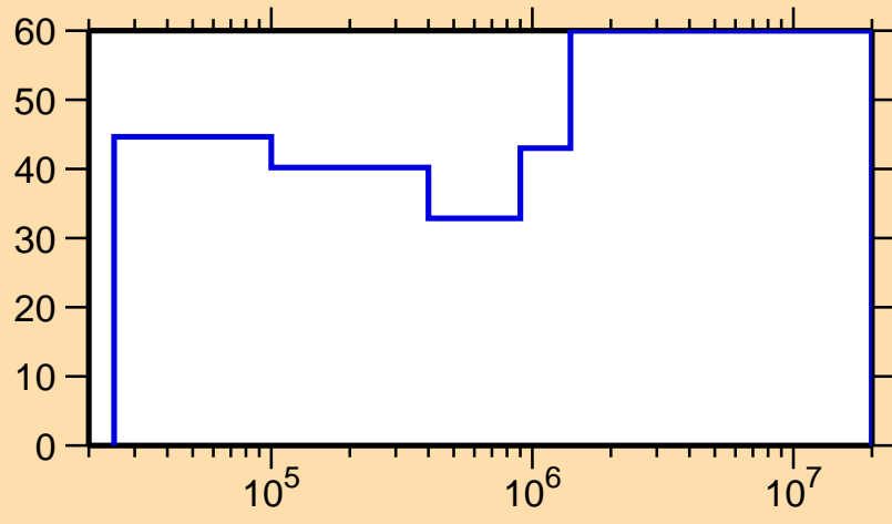
\Delta\sigma/\sigma vs. E for ^{166}\text{Tb}(n,n_1)
