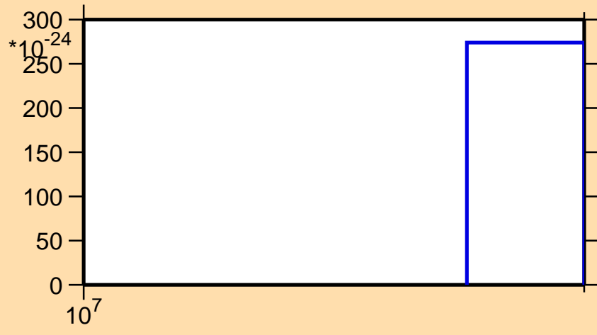
\sigma vs. E for ^{167}\text{Tb} (mt 42)
