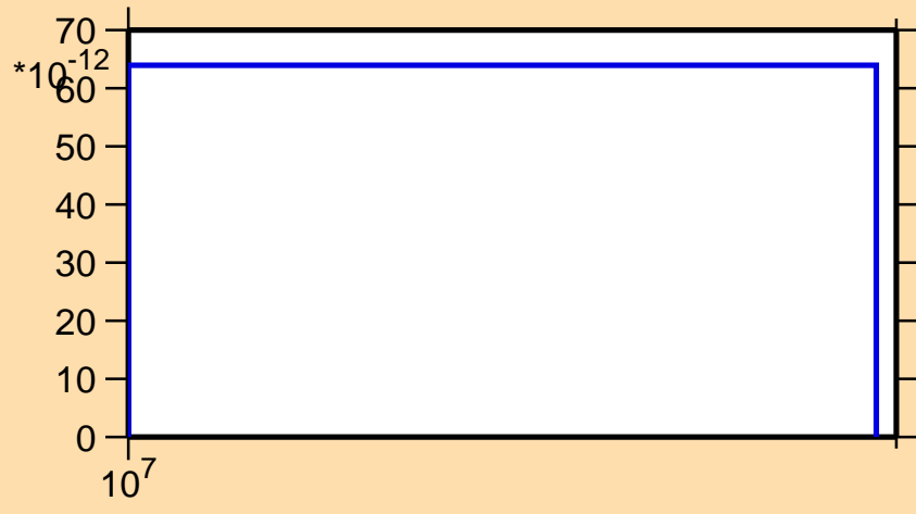
\sigma vs. E for ^{167}\text{Tb}(n,2np)
