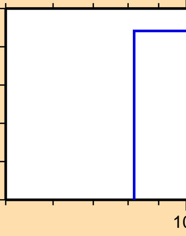
\sigma vs. E for ^{167}\text{Tb}(n,\text{nd})
