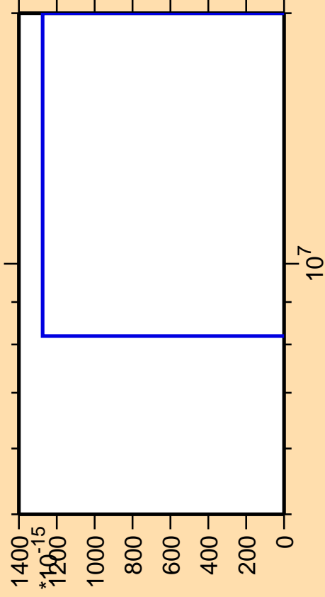
\Delta\sigma/\sigma vs. E for ^{167}\text{Tb} (mt 42)
