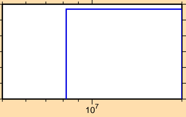
\sigma vs. E for ^{167}\text{Tb}(n,nt)
