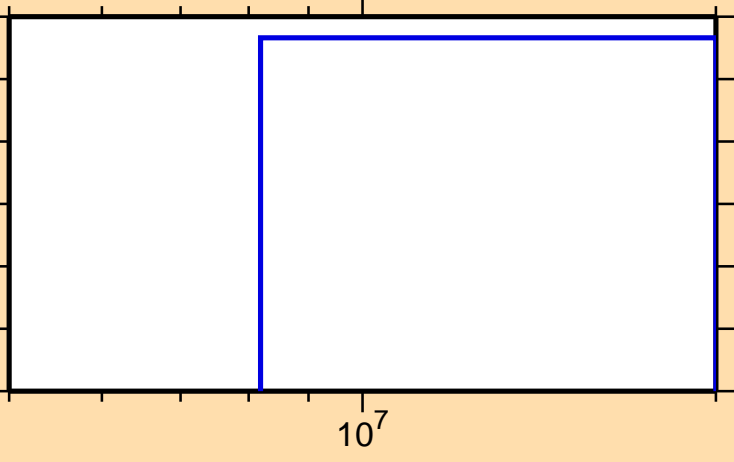
\sigma vs. E for ^{167}\text{Tb}(n,t)
