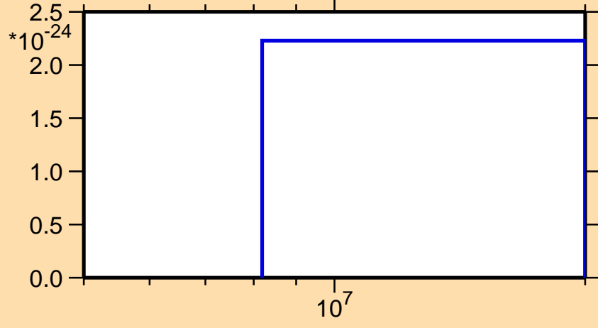
\sigma vs. E for ^{167}\text{Tb} (mt 42)
