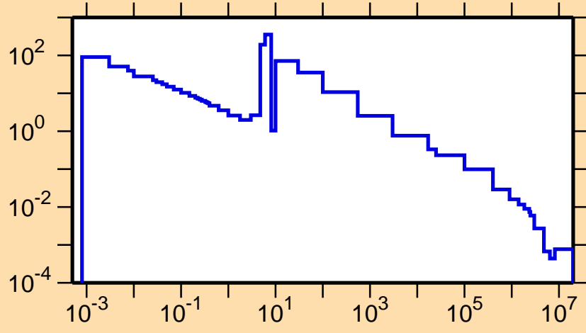
\sigma vs. E for ^{167}\text{Tb}(n,\gamma)
