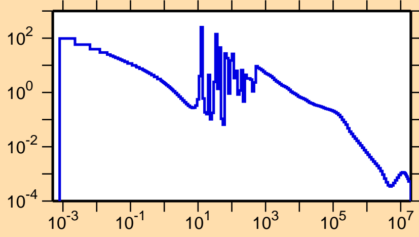
\sigma vs. E for ^{168}\text{Tb}(n,\gamma)
