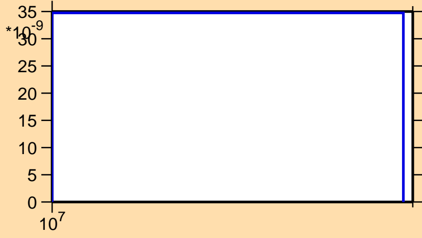
\sigma vs. E for ^{168}\text{Tb}(n,\text{nd})
