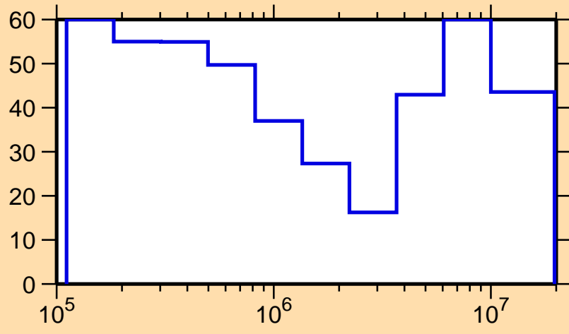
\Delta\sigma/\sigma vs. E for ^{168}\text{Tb}(n,n\text{cont.})
