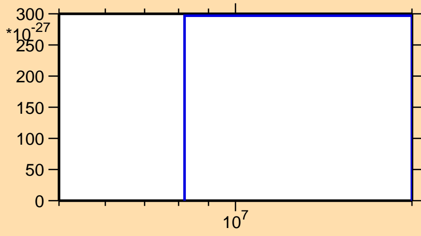
\sigma vs. E for ^{168}\text{Tb} (mt 42)
