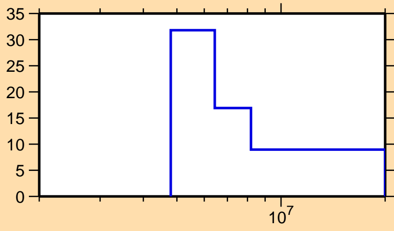
\Delta\sigma/\sigma vs. E for ^{168}\text{Tb}(n,el.)
