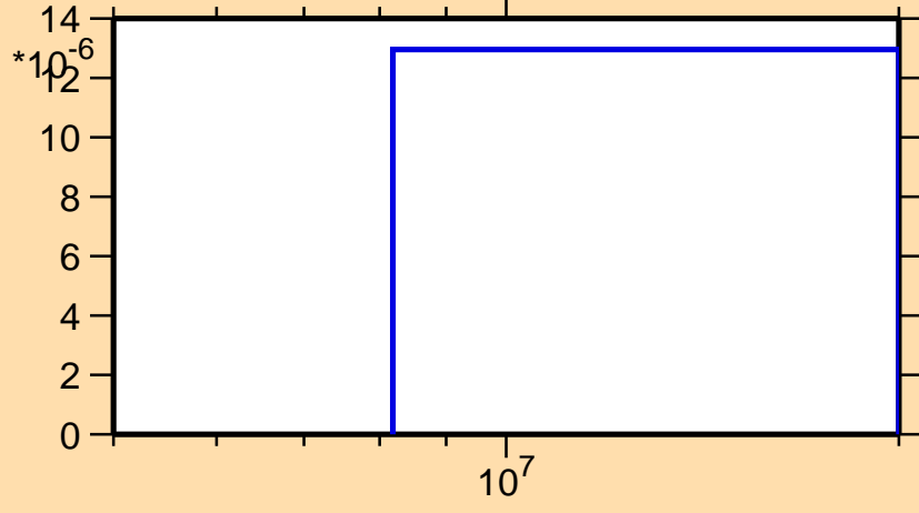
\sigma vs. E for ^{168}\text{Tb}(n,t)
