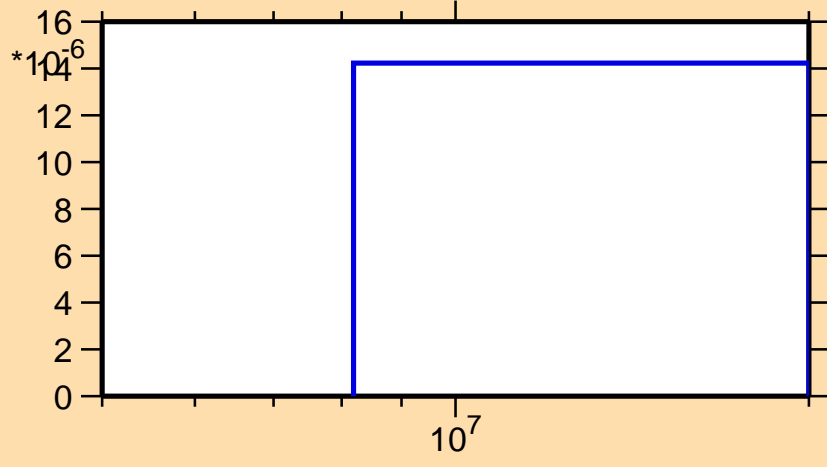
\sigma vs. E for ^{168}\text{Tb}(n,np)
