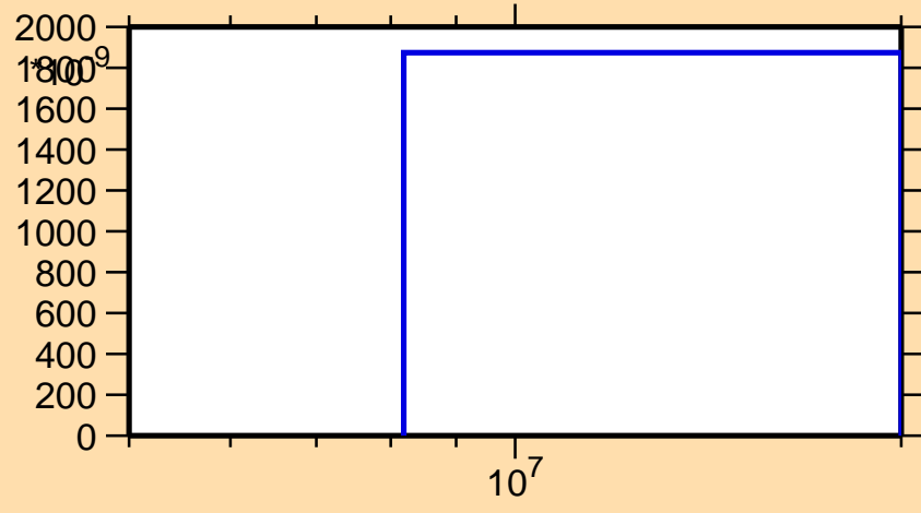
\sigma vs. E for ^{168}\text{Tb}(n,n\alpha)
