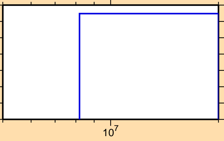
\sigma vs. E for ^{168}\text{Tb}(n,t)
