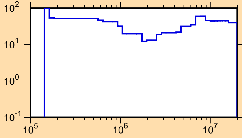
\Delta\sigma/\sigma vs. E for ^{169}\text{Tb}(n,\text{inel.})
