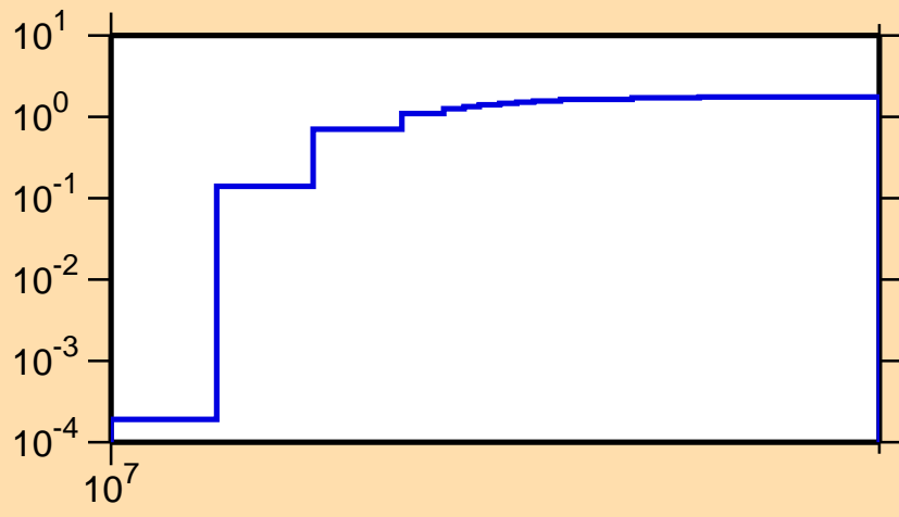
\sigma vs. E for ^{169}\text{Tb}(n,3n)
