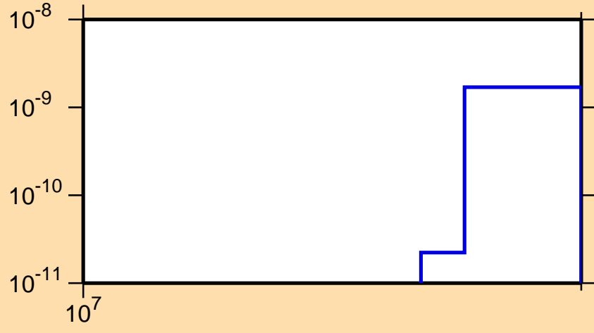
\sigma vs. E for ^{169}\text{Tb}(n,2n\alpha)
