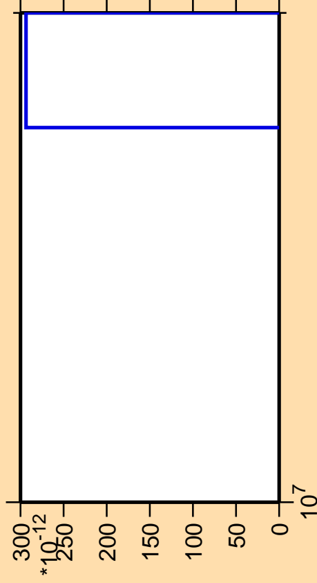
\Delta\sigma/\sigma vs. E for ^{169}\text{Tb} (mt 42)
