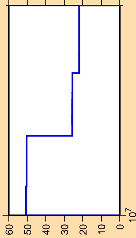
\Delta\sigma/\sigma vs. E for ^{169}\text{Tb}(n,3n)
