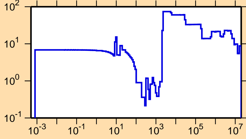
\Delta\sigma/\sigma vs. E for ^{169}\text{Tb}(n,\text{el.})
