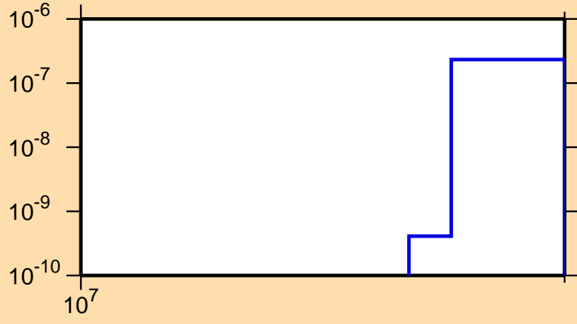
\sigma vs. E for ^{169}\text{Tb}(n,\text{nd})
