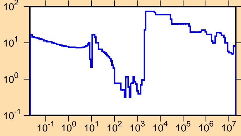
\Delta\sigma/\sigma vs. E for ^{169}\text{Tb}(n,\text{tot.})
