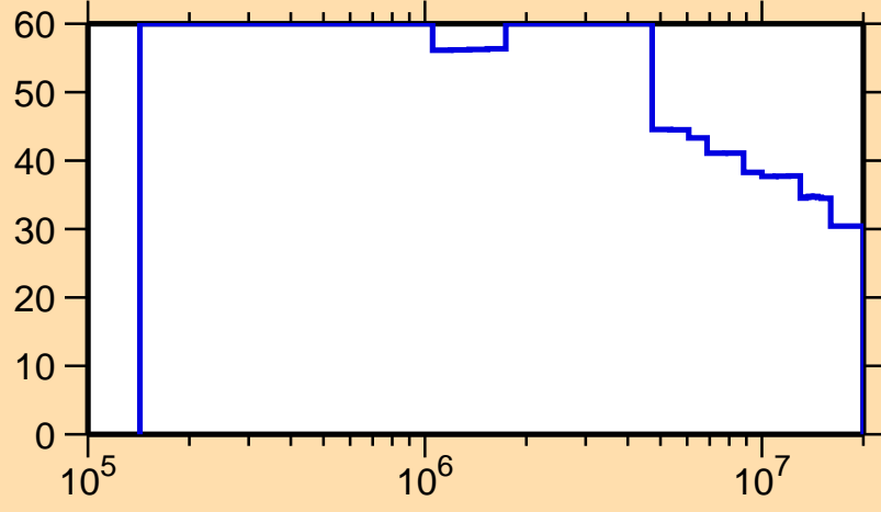
\Delta\sigma/\sigma vs. E for ^{169}\text{Tb}(n,n_1)
