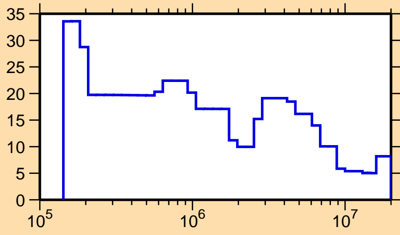
\Delta\sigma/\sigma vs. E for ^{169}\text{Tb}(n,\text{tot.})
