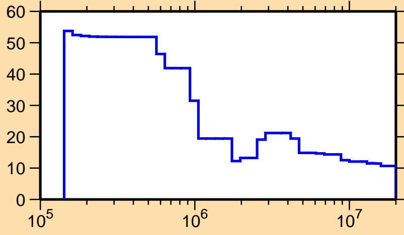
\Delta\sigma/\sigma vs. E for ^{169}\text{Tb}(n,\text{nonel.})
