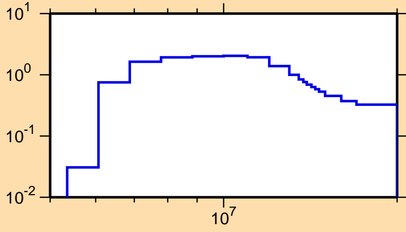
\sigma vs. E for ^{169}\text{Tb}(n,2n)
