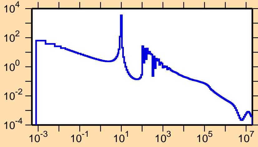
\sigma vs. E for ^{169}\text{Tb}(n,\gamma)
