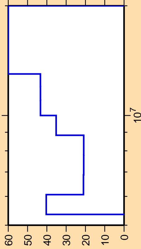
\Delta\sigma/\sigma vs. E for ^{169}\text{Tb}(n,2n)
