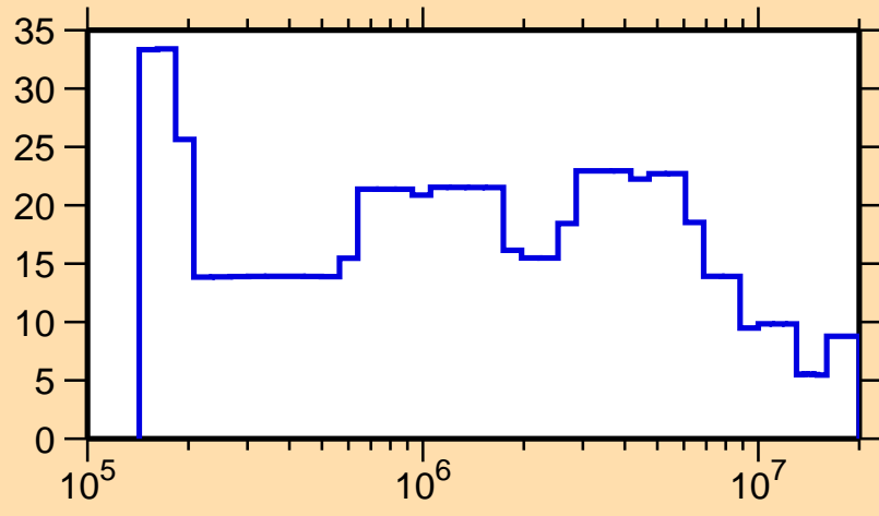
\Delta\sigma/\sigma vs. E for ^{169}\text{Tb}(n,\text{el.})
