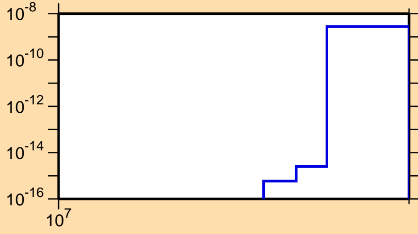
\sigma vs. E for ^{169}\text{Tb}(n,2np)
