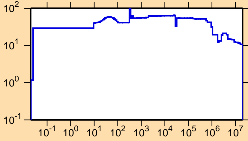
\Delta\sigma/\sigma vs. E for ^{169}\text{Tb}(n,\text{nonel.})
