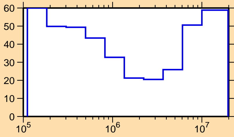
\Delta\sigma/\sigma vs. E for ^{169}\text{Tb}(n,n\text{cont.})
