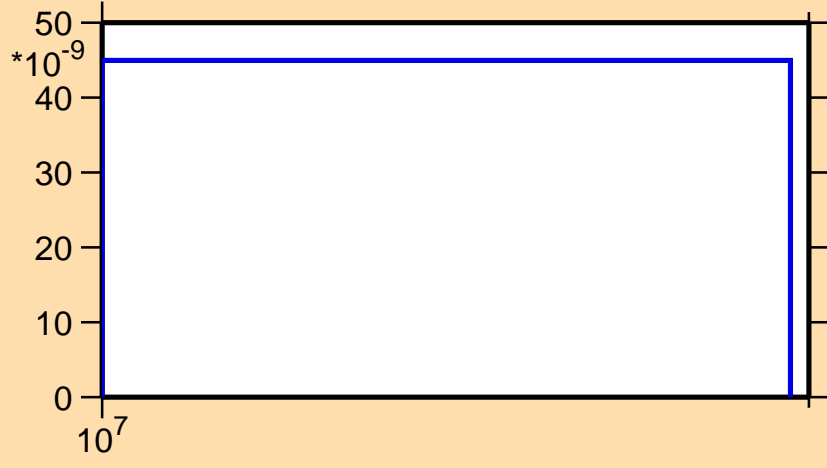
\sigma vs. E for ^{169}\text{Tb}(n,nt)
