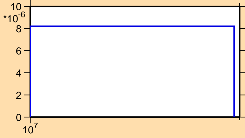
\sigma vs. E for ^{169}\text{Tb}(n,np)
