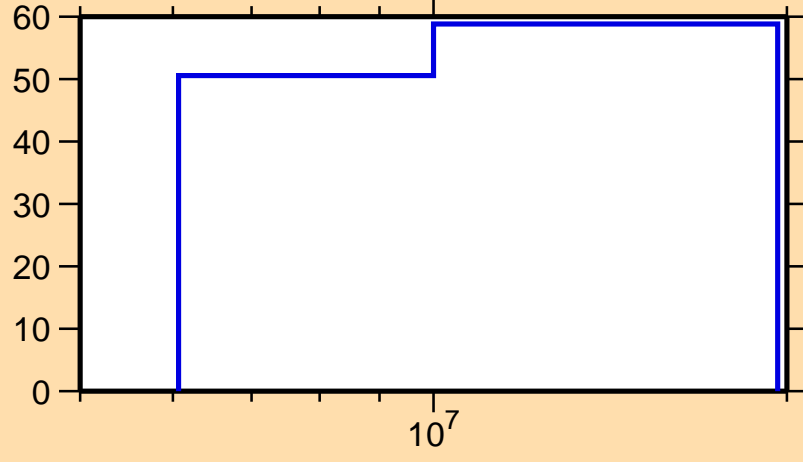
\Delta\sigma/\sigma vs. E for ^{169}\text{Tb}(n,n\text{cont.})
