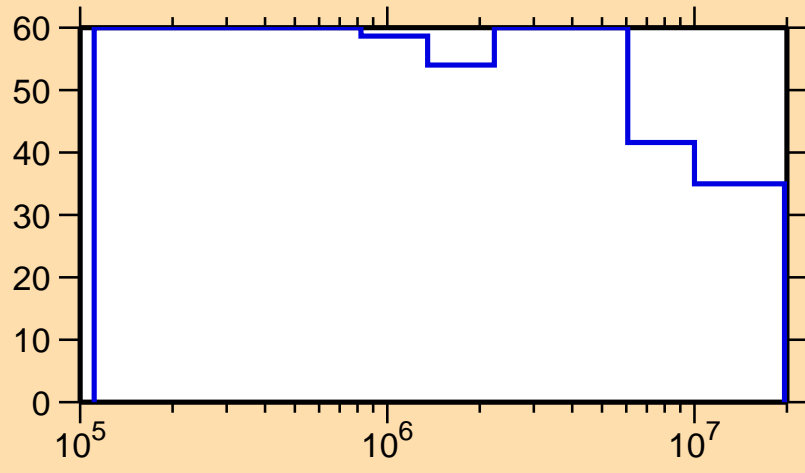
\Delta\sigma/\sigma vs. E for ^{169}\text{Tb}(n,n_1)
