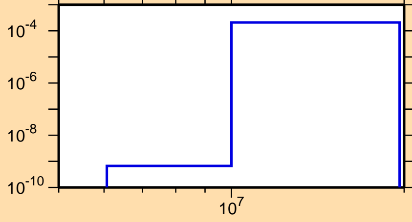
\sigma vs. E for ^{169}\text{Tb}(n,p)
