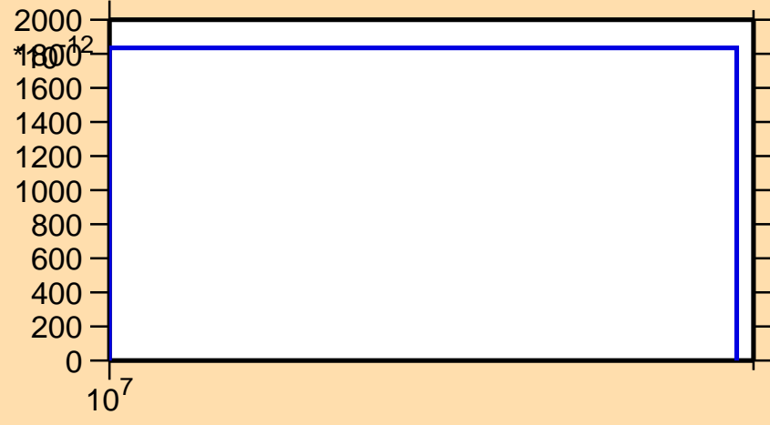
\sigma vs. E for ^{169}\text{Tb}(n,\text{nd})
