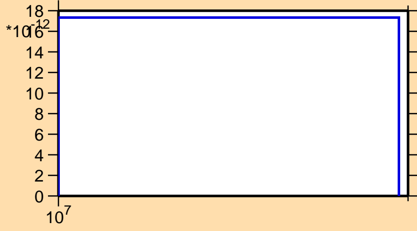
\sigma vs. E for ^{169}\text{Tb}(n,2np)
