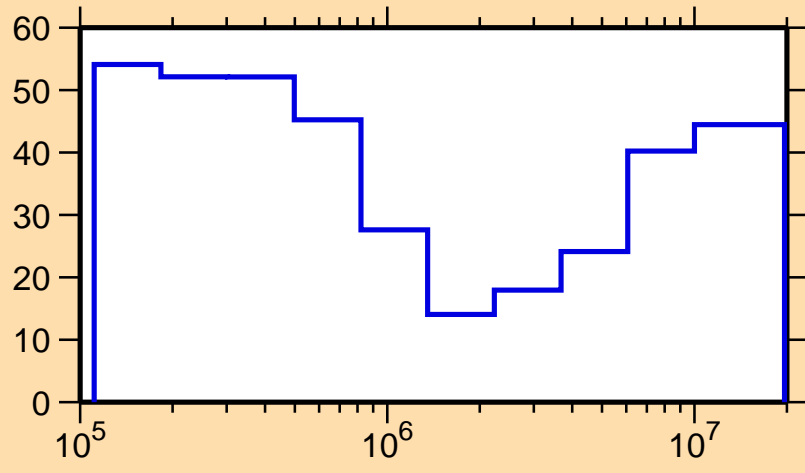
\Delta\sigma/\sigma vs. E for ^{169}\text{Tb}(n,\text{inel.})
