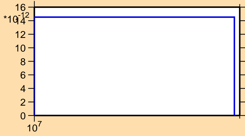
\sigma vs. E for ^{169}\text{Tb}(n,2n\alpha)
