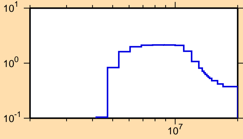
\sigma vs. E for ^{170}\text{Tb}(n,2n)
