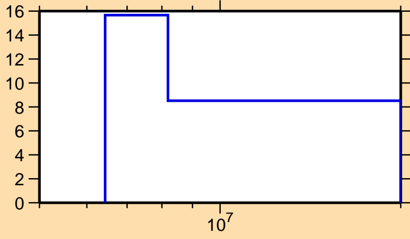
\Delta\sigma/\sigma vs. E for ^{170}\text{Tb}(n,el.)
