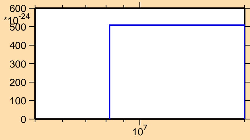
\sigma vs. E for ^{170}\text{Tb} (mt 42)
