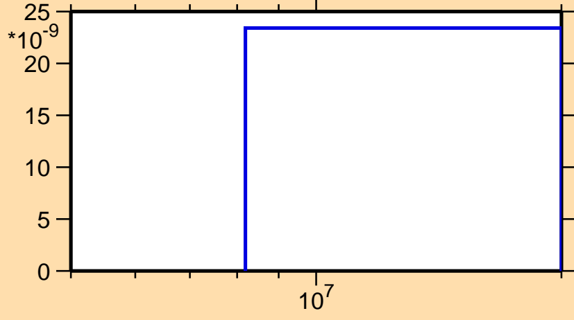
\sigma vs. E for ^{170}\text{Tb}(n,\text{nd})
