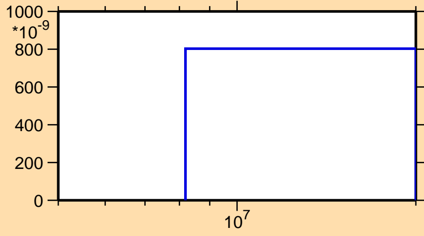
\sigma vs. E for ^{170}\text{Tb}(n,n\alpha)
