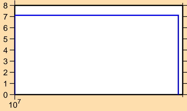
\Delta\sigma/\sigma vs. E for ^{88}\text{Tc}(n,\text{tot.})
