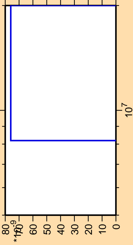
\Delta\sigma/\sigma vs. E for ^{88}\text{Tc}(n,nt)
