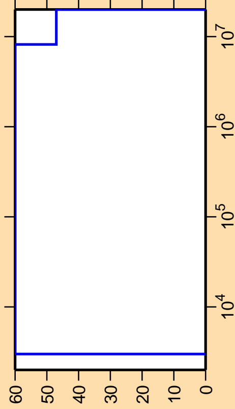
\Delta\sigma/\sigma vs. E for ^{88}\text{Tc}(n,ncont.)
