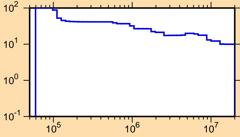
\Delta\sigma/\sigma vs. E for ^{89}\text{Tc}(n,n_1)
