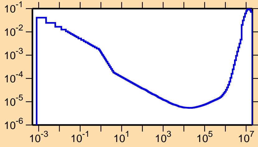
\sigma vs. E for ^{89}\text{Tc}(n,\alpha)
