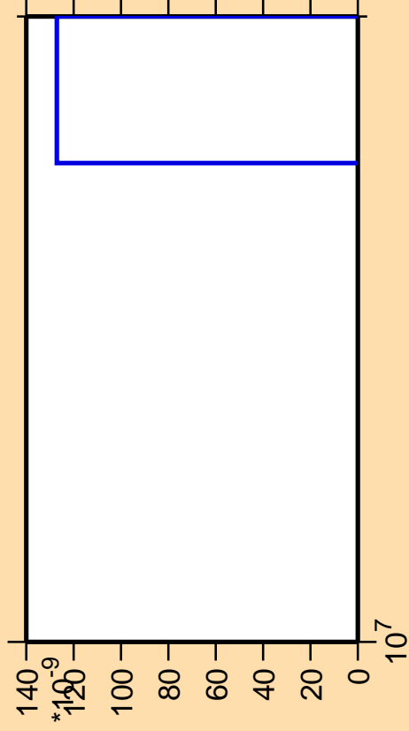
\Delta\sigma/\sigma vs. E for ^{89}\text{Tc}(n,nt)
