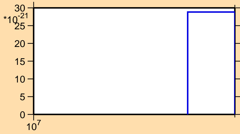
\sigma vs. E for ^{89}\text{Tc}(n,nt)
