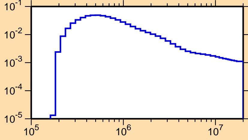
\sigma vs. E for ^{89}\text{Tc}(n,n_2)
