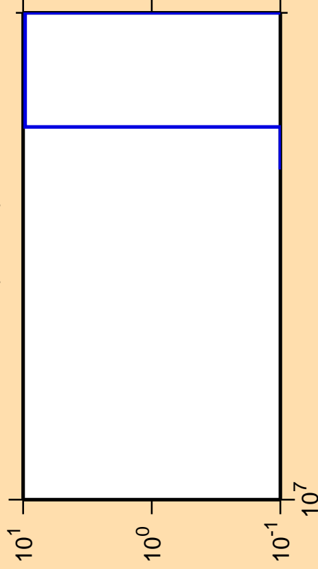
\Delta\sigma/\sigma vs. E for ^{89}\text{Tc} (mt 34)
