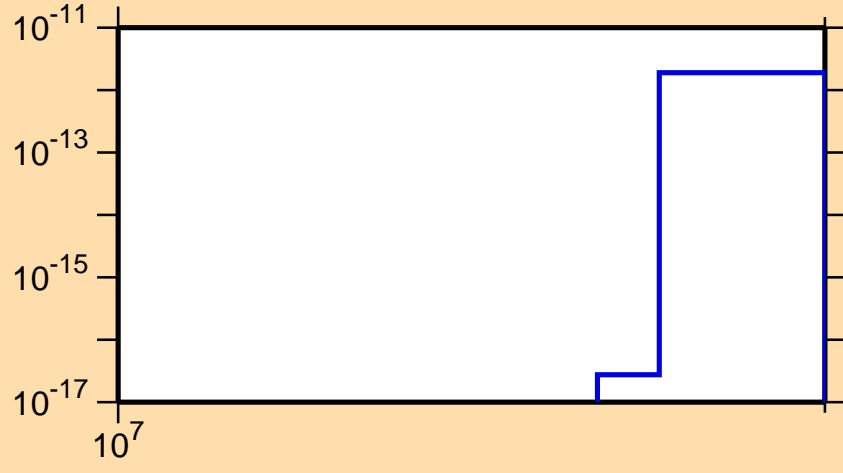
\sigma vs. E for ^{89}\text{Tc} (mt 34)
