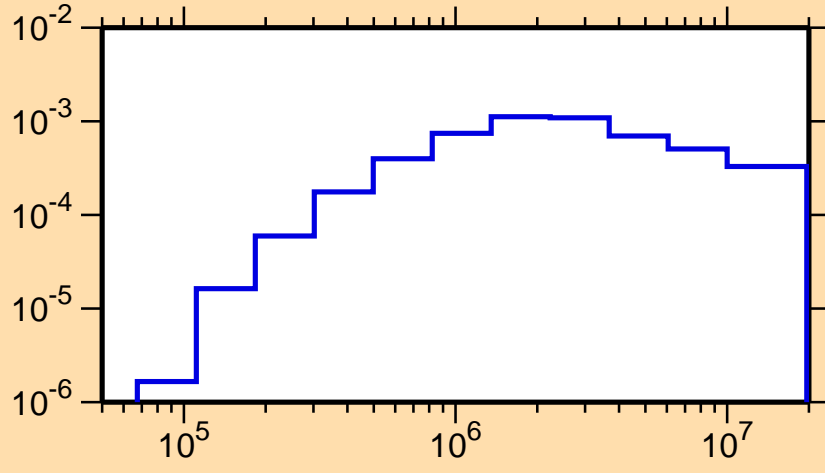
\sigma vs. E for ^{89}\text{Tc}(n,n_1)
