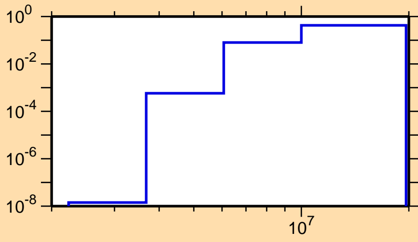
\sigma vs. E for ^{89}\text{Tc}(n,np)
