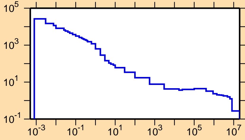
\sigma vs. E for ^{89}\text{Tc}(n,p)
