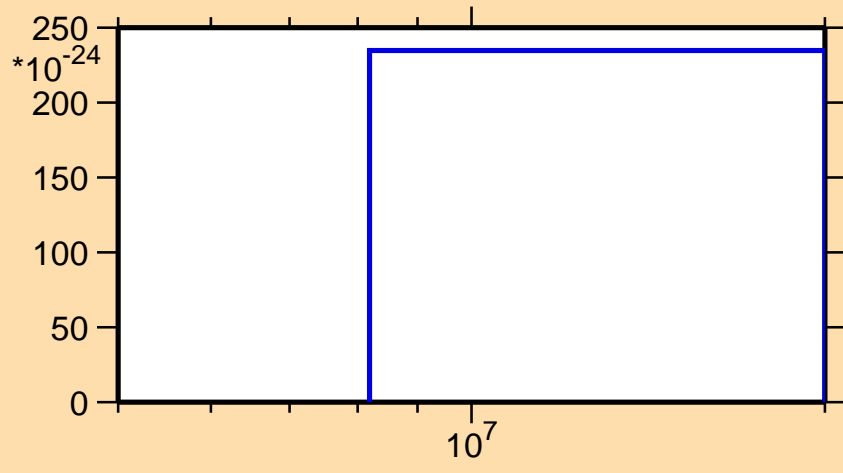
\sigma vs. E for ^{89}\text{Tc}(n,nt)
