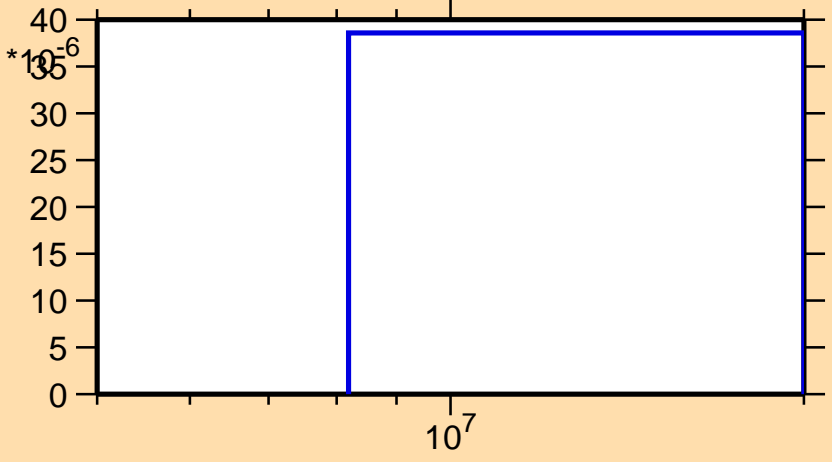
\sigma vs. E for ^{89}\text{Tc}(n,t)
