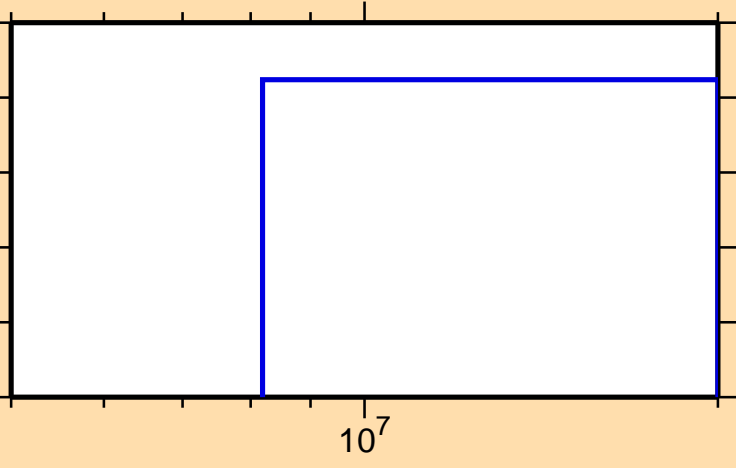
\sigma vs. E for ^{89}\text{Tc} (mt 45)
